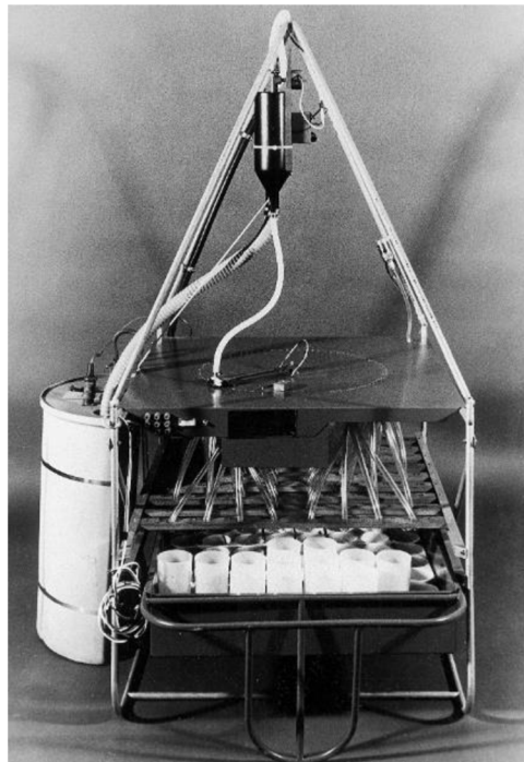
Obr. 17. Sampler US PS-69 [9]
