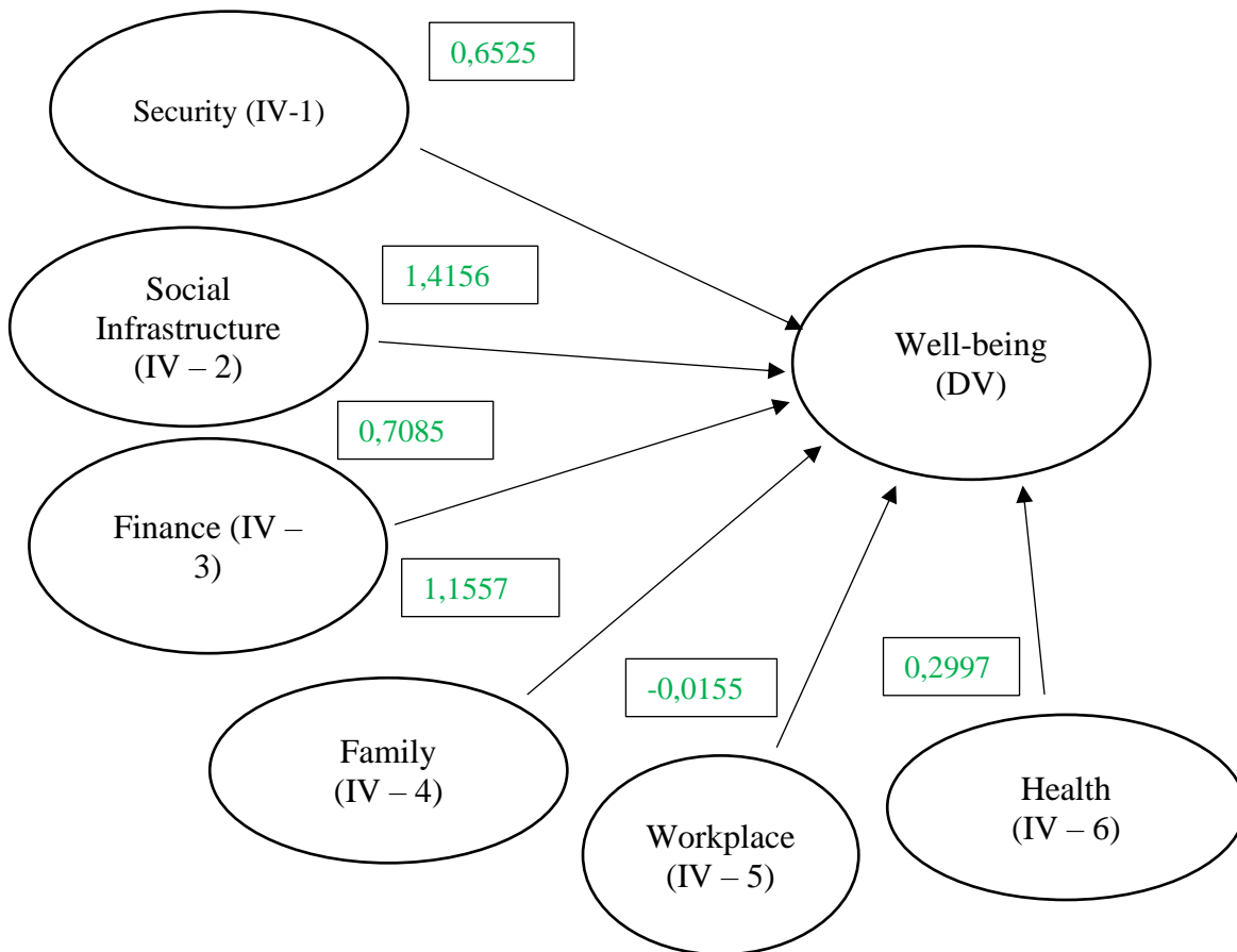
Figure 10: Final Model
