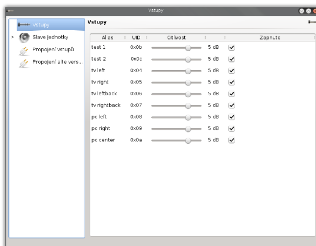
Obr. 5.12: Widget "Vstupy"
