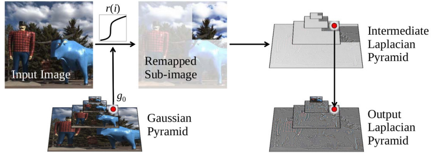
Figure 3.2: Local Laplacian Filters algorithm overview. Image taken from authors’s paper [22, p. 5].
