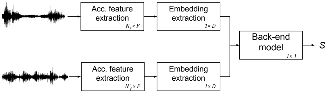
Figure 1.1: Typical speaker verification pipeline. The subscripts in the blocks correspond to the dimensionality of the output of the current stage.
