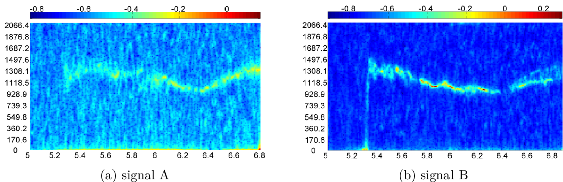
Fig. 6.5: Enhanced PDV data ( x -axis: time, y -axis: frequencies).
