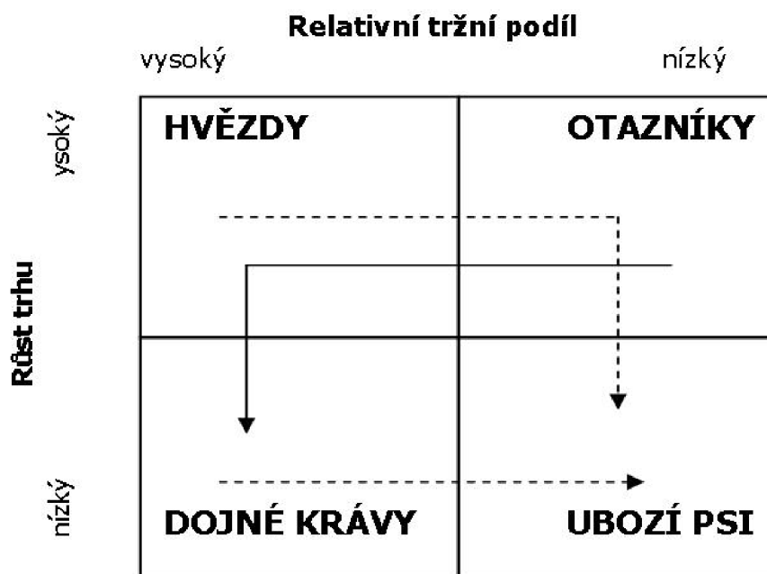
Obr.12 Matice BCG[9]
