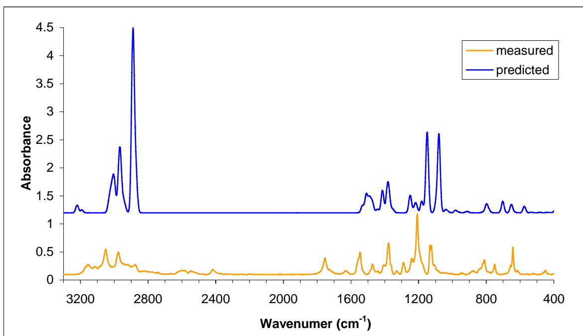
Fig. 38 The comparison of measured (SH) and predicted (DFT/6-31*) IR spectra of NC 1 H-Cl
