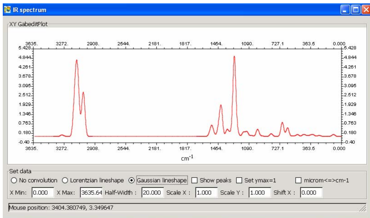
Fig. 28 The visualisation of IR spectrum in Gabbit
