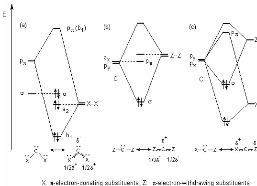
Fig. 10 Perturbation orbital diagrams showing the influence of the mesomeric effects
