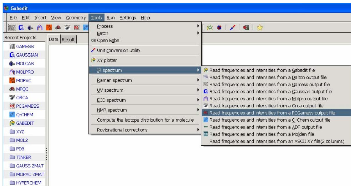
Fig. 27 Reading of IR spectrum in Gabbit
