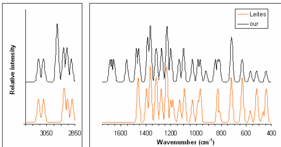
Fig. 42 The comparison of measured spectra of \text{NC}_1
