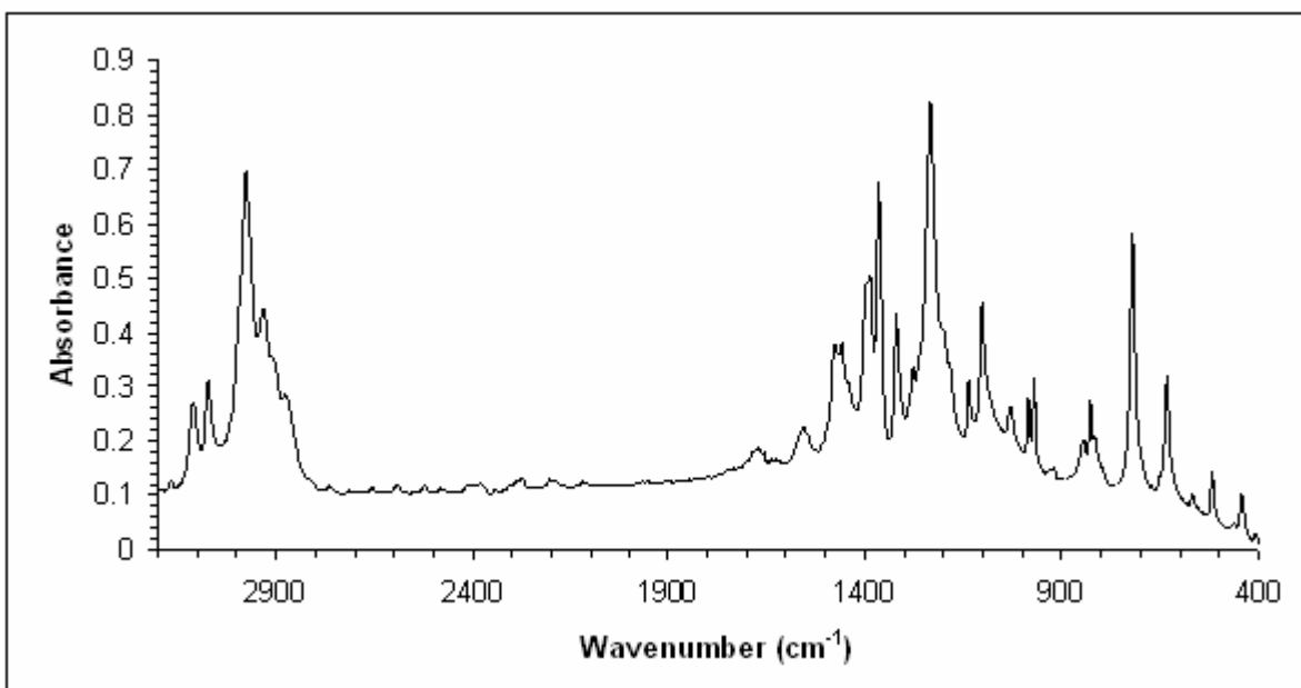
Fig. 41 The measured IR spectrum of \text{NC}_1 (Nujol, KBr) \nu ( \text{cm}^{-1} ): 444 (vw), 519 (vw), 567 (vw), 633(w), 719 (s), 816 (w), 827 (w), 847 (w), 922 (vw), 970 (w), 986 (w), 1031 (w), 1101 (m), 1136 (w), 1202 (m), 1234 (vs), 1277 (m), 1319 (m), 1366 (vs), 1387 (s), 1458 (m), 1476 (m), 1555 (w), 1657 (w), 1672 (w), 1686 (w), 2876 (w), 2909 (m), 2932 (m), 2976 (vs), 3073 (w), 3109 (w)
