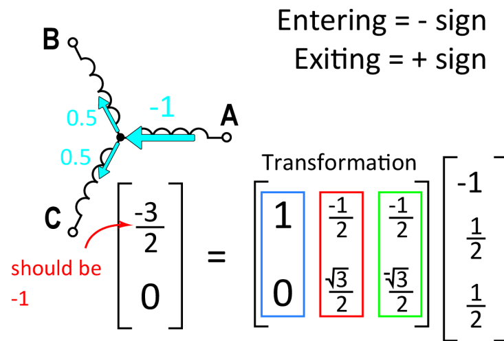
Figure 97: Why multiplier in the transformation
