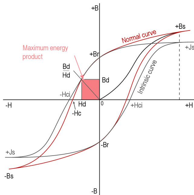
Figure 89: Normal curve
