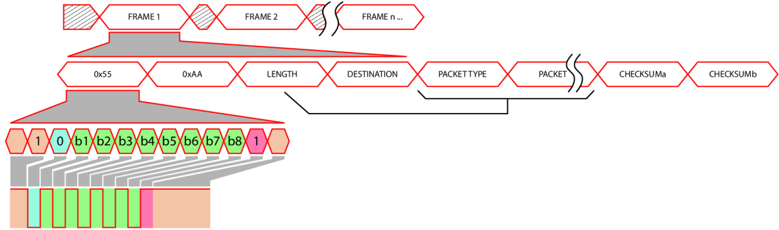
Figure 72: Communication protocol structure
