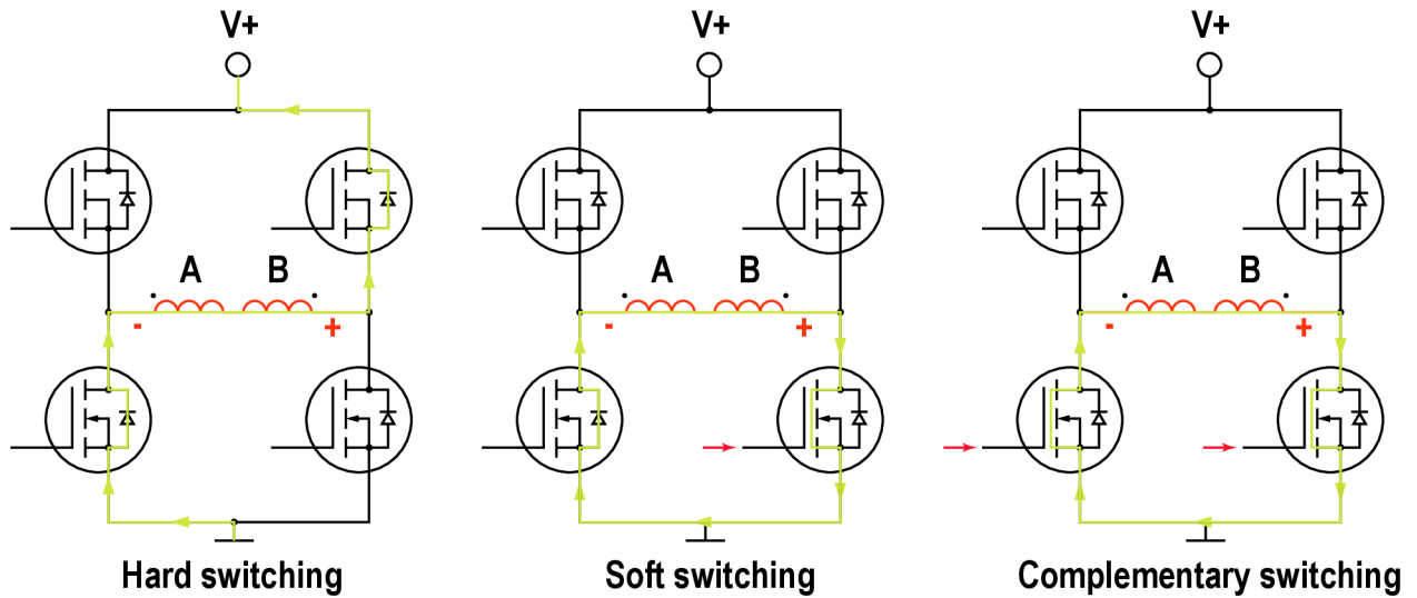
Figure 33: Switching options during dead time
