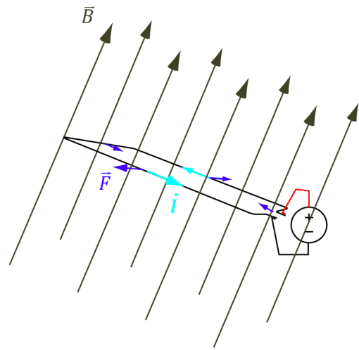
Figure 17: No torque
