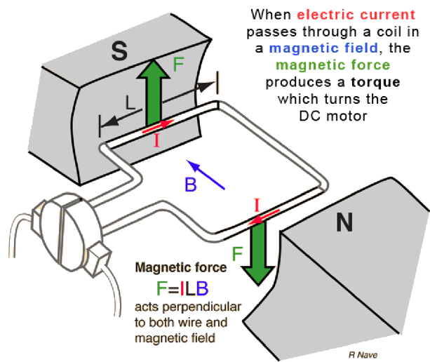
Figure 14: Magnetic effect in a motor 2
