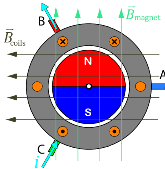
Figure 28: Rotor and stator fields inside motor
