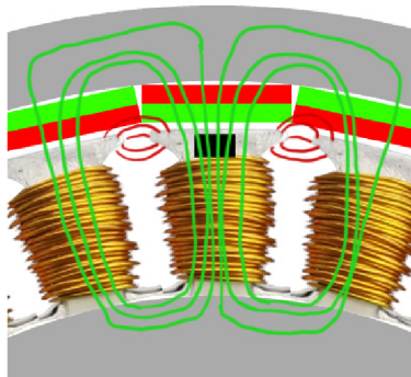
Figure 12: Leakage flux
