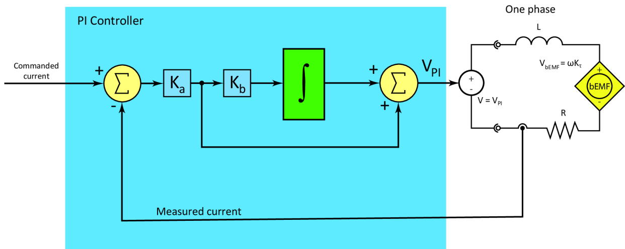
Figure 50: Current loop
