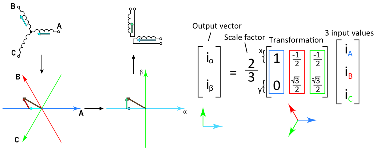
Figure 96: Clarke transformation
