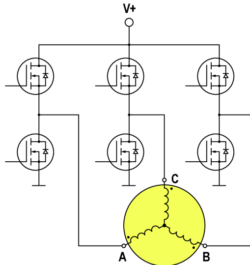
Figure 32: Switching elements on the phases
