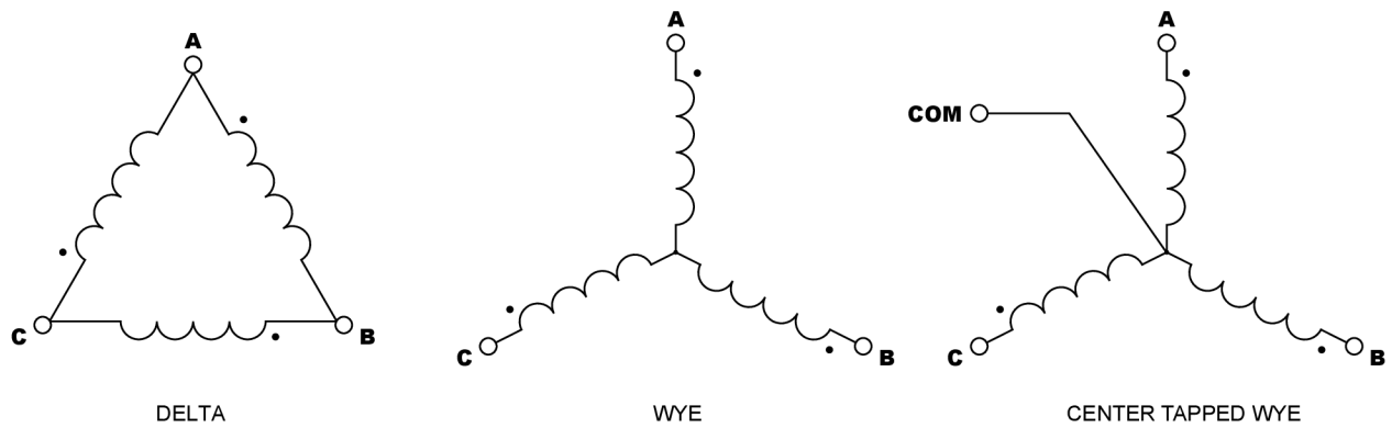
Figure 10: Configurations of three motor phases
