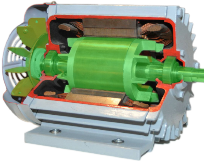
Figure 1: Industrial motor
