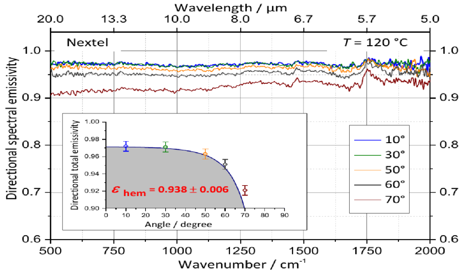
Figure 12: Angular distribution of the directional spectral emittance of Nextel Velvet Black 811-21 measured at a temperature of 120 °C [13].
