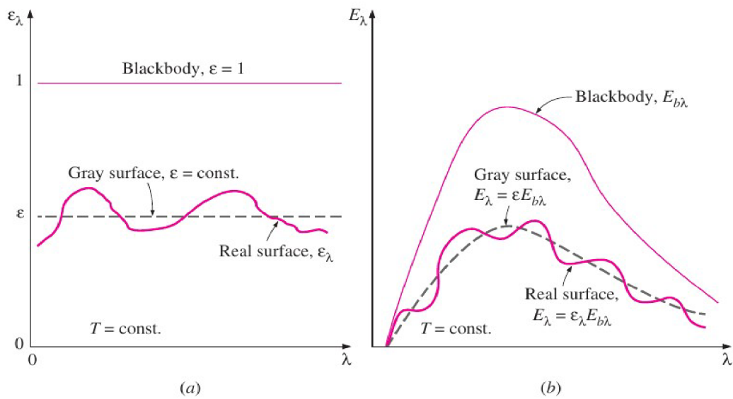
Figure 10: Comparison of the emissivity (a) and emissive power (b) of a real surface with those of a gray surface and a blackbody at the same temperature [7].
