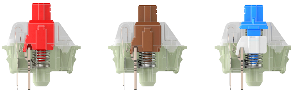
Fig. 11: Cutaway view of Cherry MX switches. From left to right: linear, tactile and clicky. [30–32].
