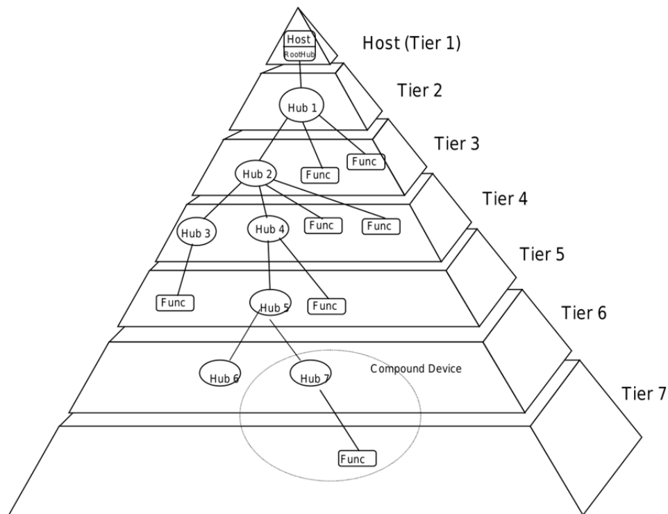
Fig. 21: USB bus topology [52].
