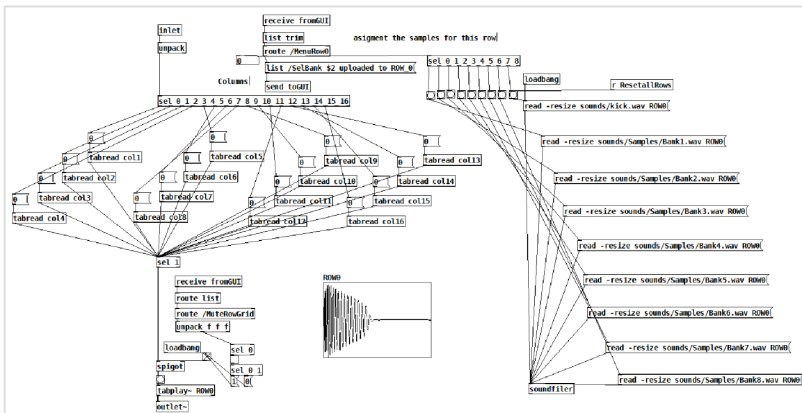
obr. 3-4: pd row0
