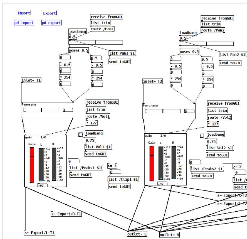
obr. 3-17: Mix track1 a track 2
