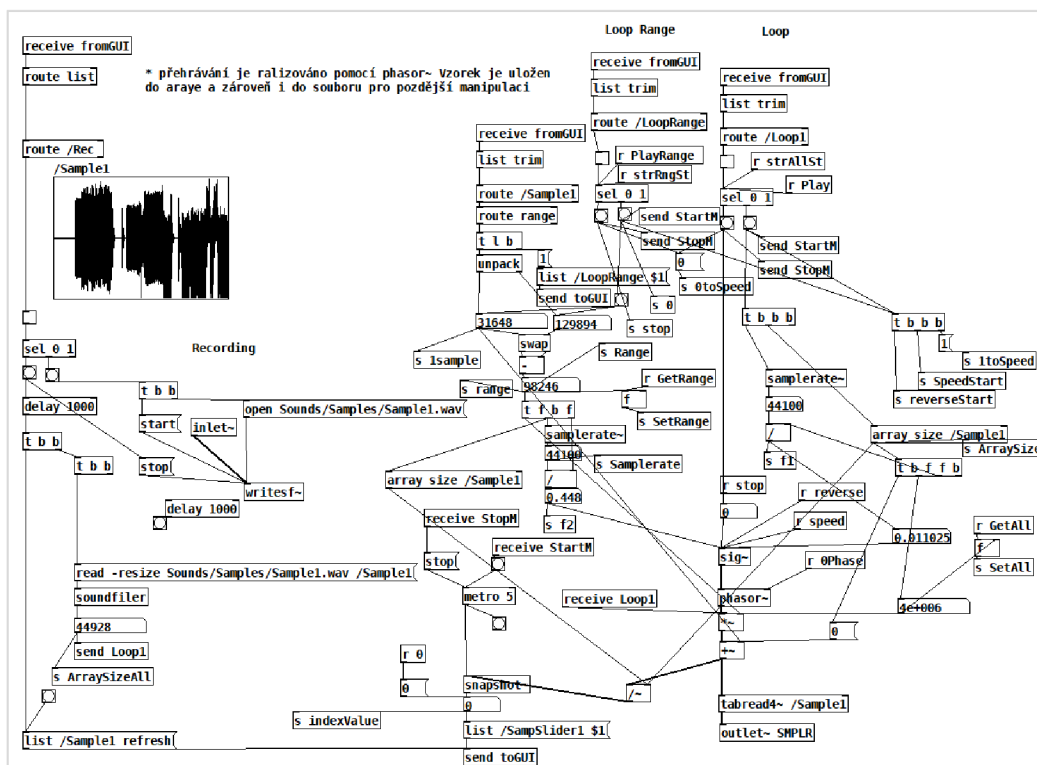
obr. 3-14: Sampler
