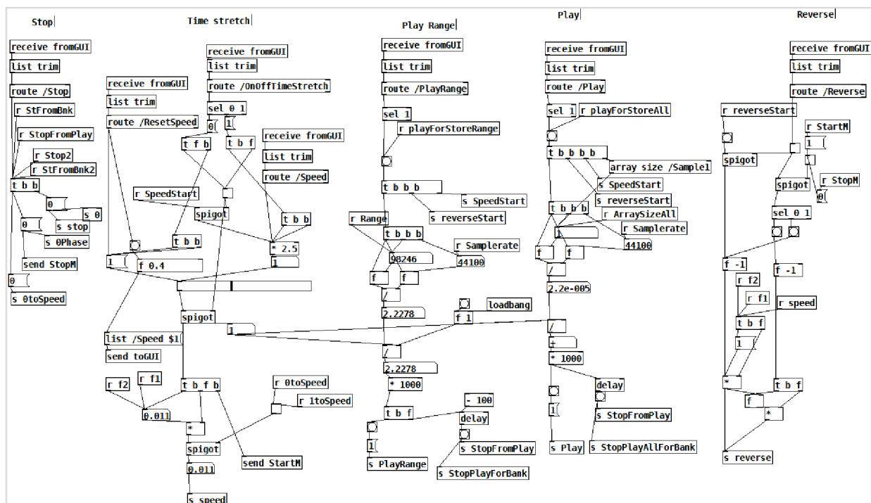
obr. 3-15: Sampler
