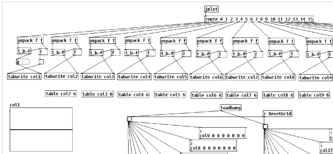
obr. 3-3: pd GridSet
