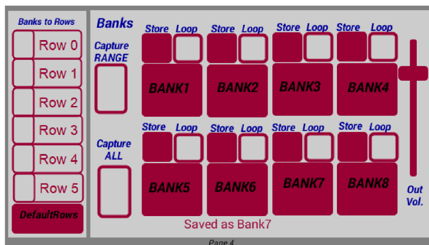
obr. 2-7: Banks
