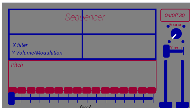
obr. 2-5: Sequencer
