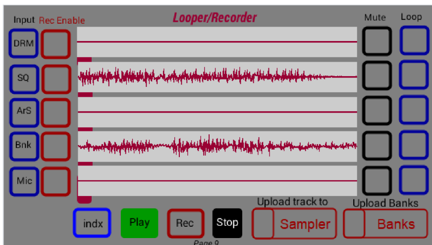
obr. 2-12: Looper/Recorder
