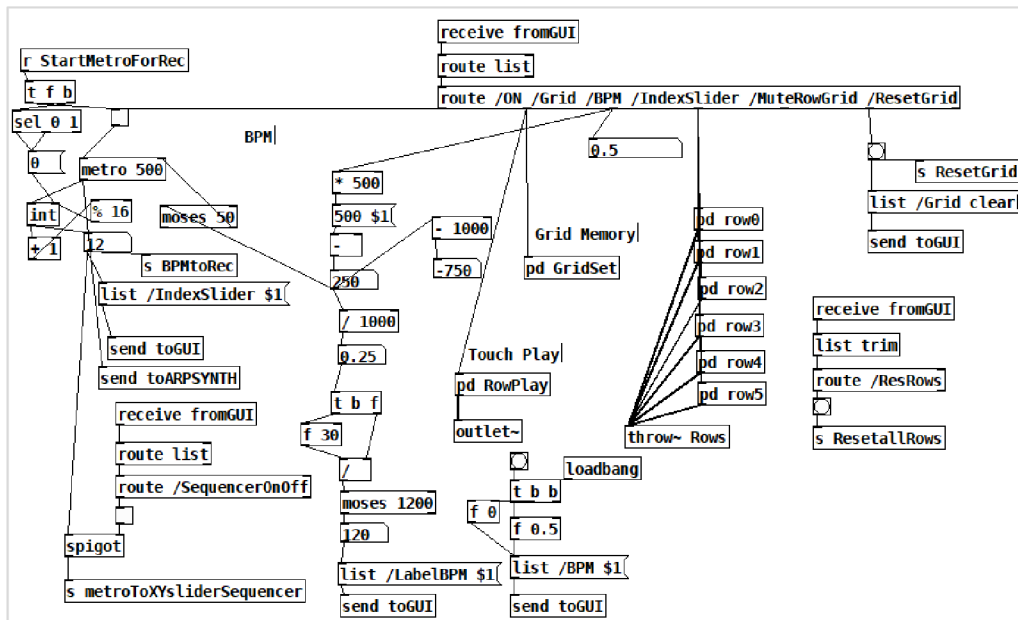
obr. 3-2: pd DrumMachine
