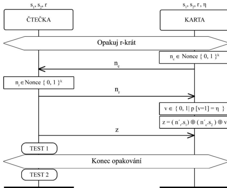
Obr. 4.10 HB+ protokol
