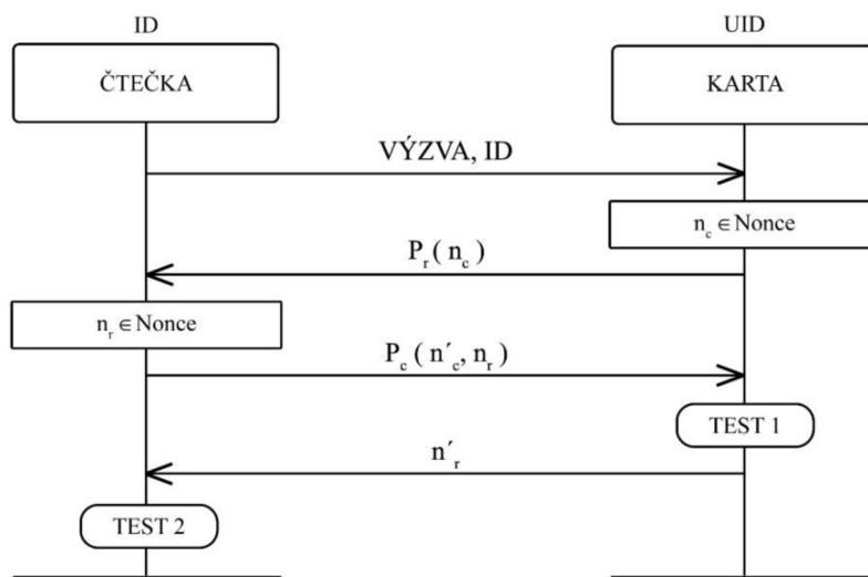
Obr. 4.14 Needham-Schroeder
