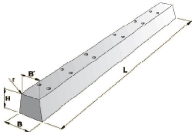
Obr. 3.2.6 Pražec B91S [2]
