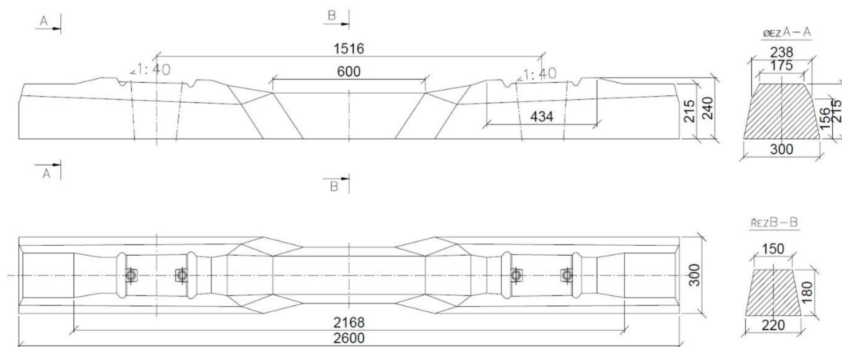
Obr. 3.2.5 Pražec B91S [4]
