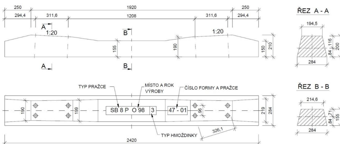
Obr. 3.2.4 Pražec SB 8P [4]
