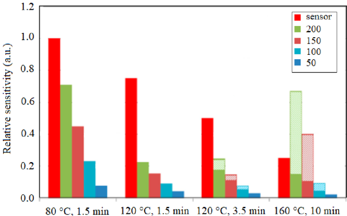
Fig. 45 Experimental relative sensitivities of repaired sensors (red columns). Calculated relative active (sensitivity) areas (full columns) and deformation contribution areas (hatched columns). Differently coloured columns indicate the contributions below the defined threshold level.
