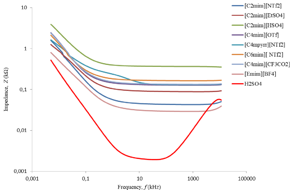
Fig. 27 Dependence of impedance on frequency of chosen ionic liquids, H 2 SO 4 is added for comparison.
