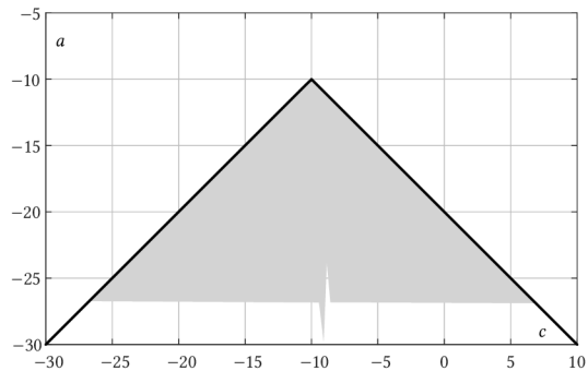
Obr. 2: b = -20, m = 2, l = 1
