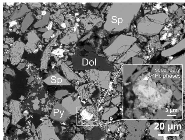
Fig. 1. Scanning electron micrograph in back-scattered electrons (SEM-BSE) of the Tl-rich sulfide concentrate used in the pot trial. Phase abbreviations: Sp – sphalerite (ZnS); Py – pyrite (FeS 2 ); Dol – dolomite (CaMg(CO 3 ) 2 ).
