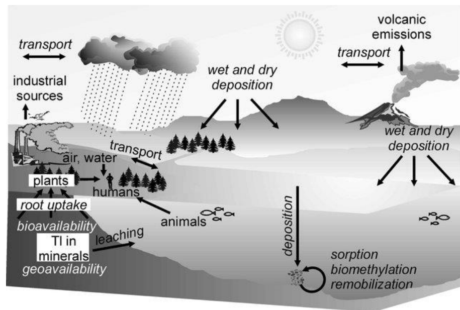
Figure 2. The main sources and geochemical processes that control Tl in the environment (source: Migaszewski and Gałuszka, 2021)
