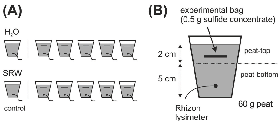
Fig. 2. The pot trial setup with bags containing sulfide concentrate – Tl/trace element source (A). Deionized H 2 O (H 2 O) and synthetic rainwater (SRW) were used for peat watering. Pots without bags were used as a control variant. Location of the bag, Rhizon pore solution sampler and peat segments sampled at the end of the concentrate incubation (12 weeks) (B).
