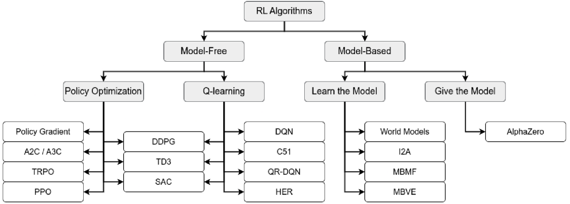
Figure 3.6: Taxonomy of RL algorithms derived from [43]; Policy Gradient[44], A2C/A3C[45], TRPO[46], PPO[47], DDPG[48], TD3[49], SAC[50], DQN[51], C51[52], QR-DQN[53], HER[54], World Models[55], I2A[56], MBMF[57], MBVE[58] and AlphaZero[59]
