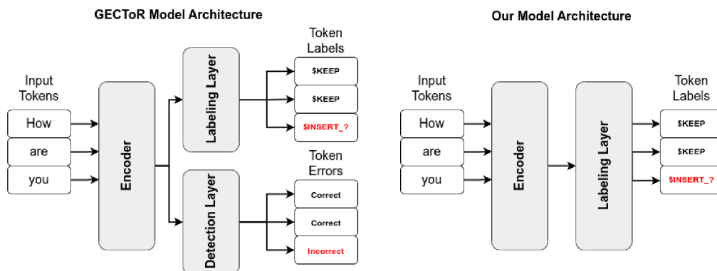
Figure 4.4: Comparison between GECToR’s and our model architectures
