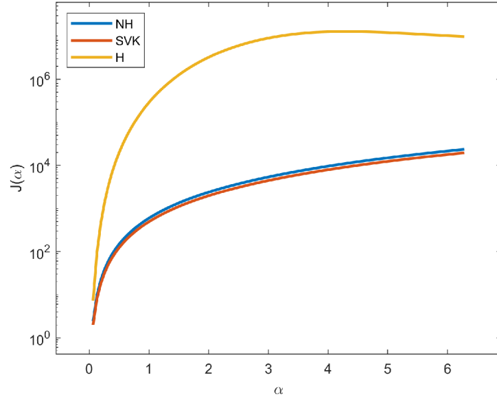
Figure 3.5: The comparison of exact energies.
