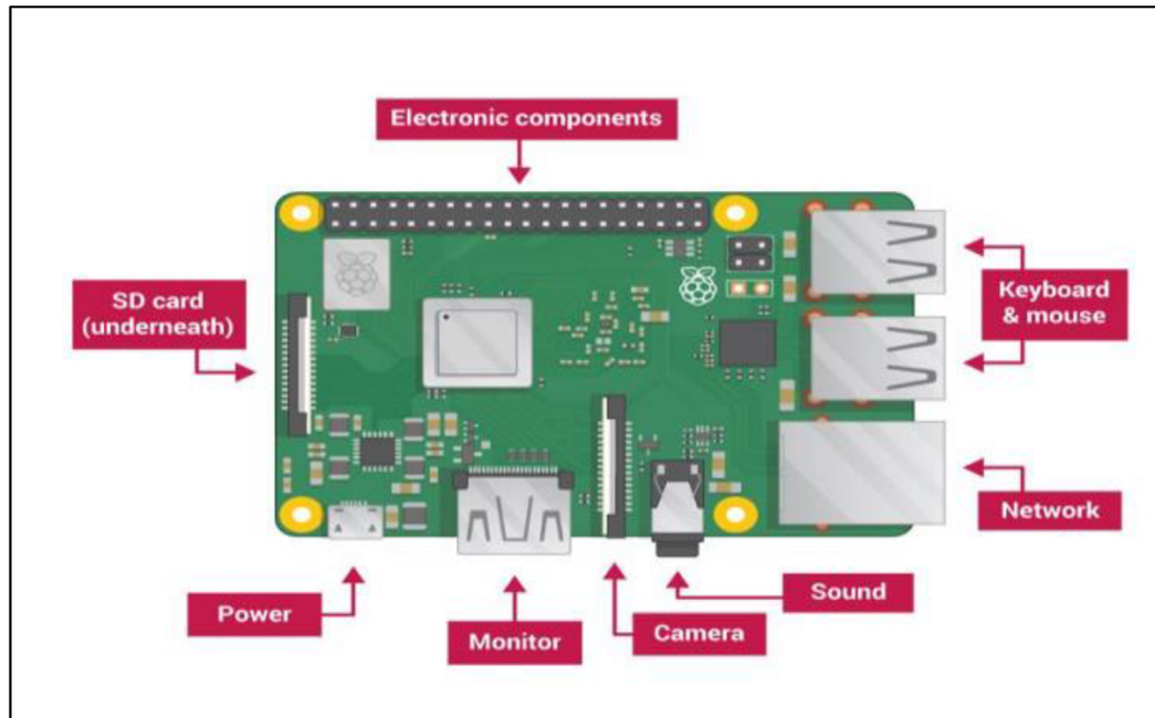
Figure 2 Raspberry Pi ports label diagram. Reprinted from Raspberry Pi projects (Jain, A., et Al., 2019)
