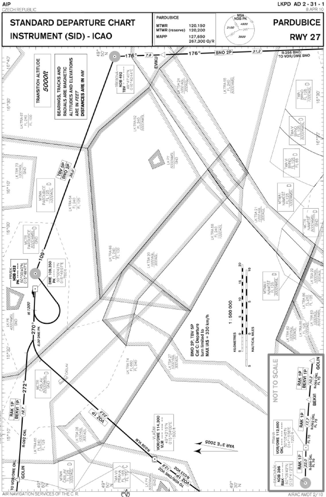
Obr. H – SID RWY 27 LKPD [2]
