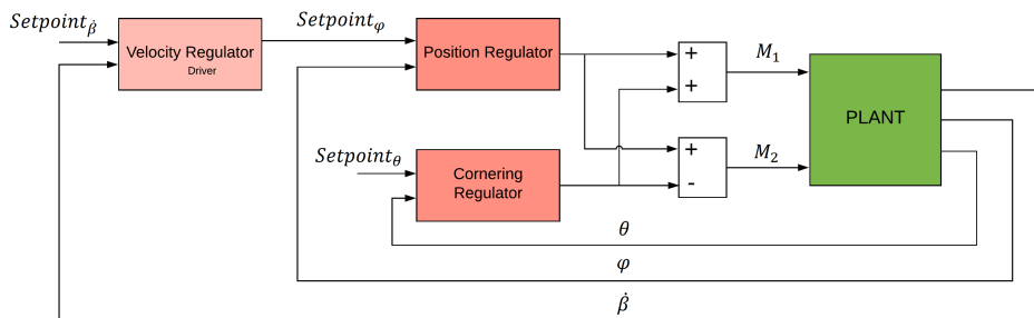
Figure 5.4: Block diagram of the cornering regulator and regulator for stabilization
