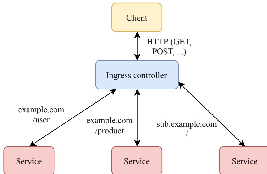
Figure 3.6: Kubernetes Ingress controller works on the application level of the network model. This allows routing of the HTTP requests to different Services based on hostname or path they are requesting.
