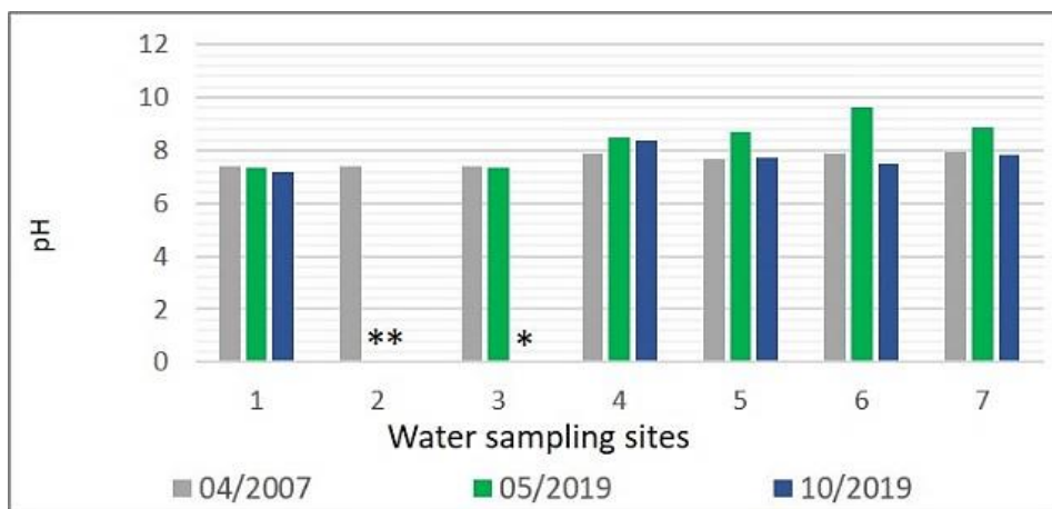
Figure 6.3: pH along the monitored profile of the pond system (April 2007, May 2019, and October 2019) (* not sampled).
