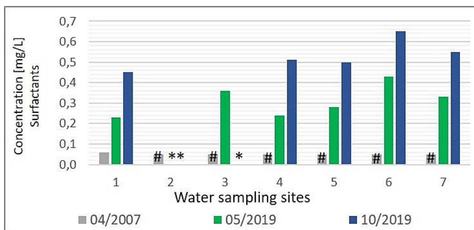
Figure 6.7: Surfactant concentration along the observed profile of the pond system (April 2007, May 2019, and October 2019) (* not sampled, # values <0.05).
