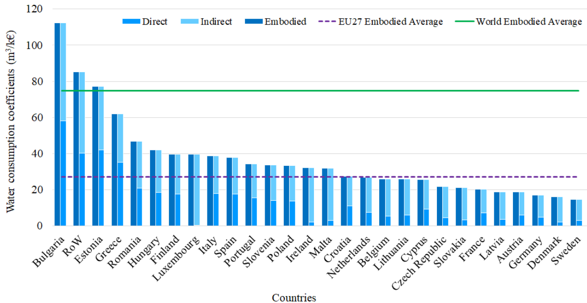
Figure 16 Direct and Indirect EWCC
