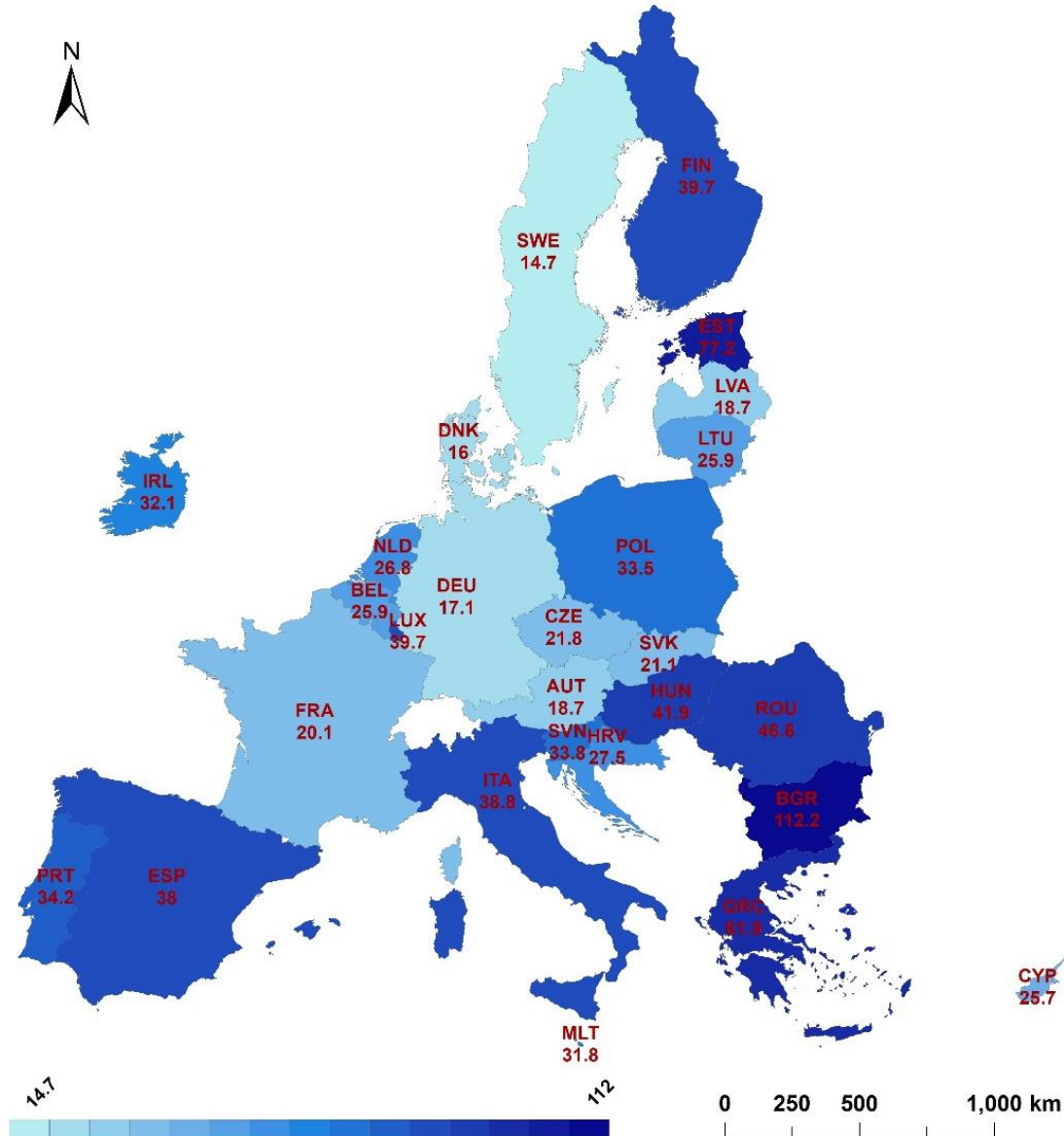
Figure 15 EWCC of the EU27 (m 3 /k€)
