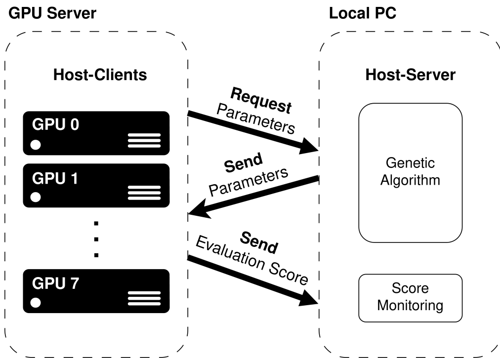
Fig. 5.2: Principle of GA distribution on multiple GPUs
