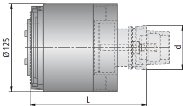
Obr. 9 Jednotka UAS-125-Z-12 [20]
