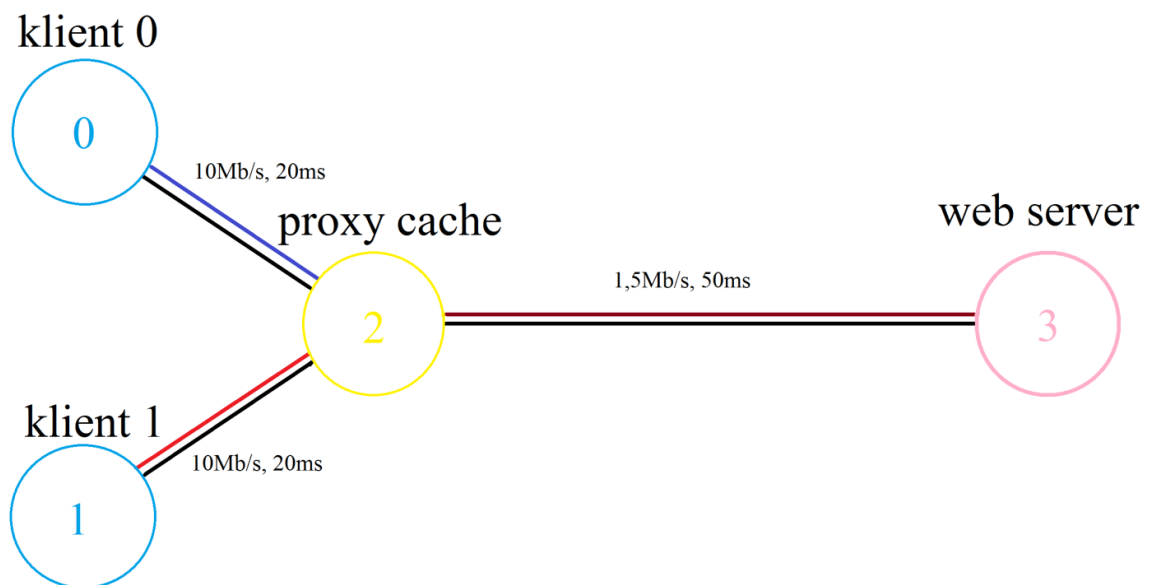
Obr. 1: Schéma simulace.
