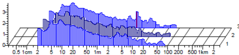
Spectrogram Mass
