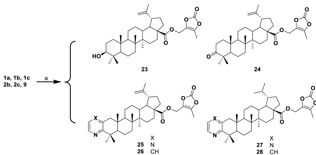
Scheme 4. Synthesis of medoximil prodrugs 23–28. Reagents and conditions: a) 4-(chloromethyl)-5-methyl-1,3-dioxol-2-one, \text{KI} , \text{K}_2\text{CO}_3 , acetone, r.t.
