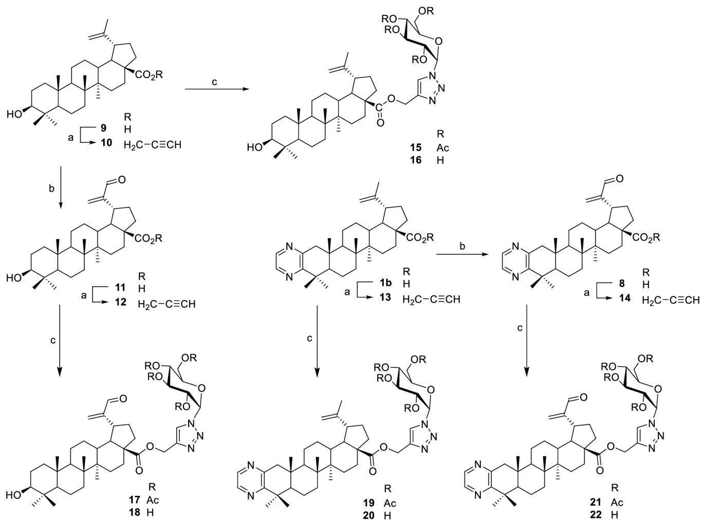
Scheme 3. Preparation of triterpenoid conjugates with glucose. Reagents and conditions: a) propargyl bromide, \text{K}_2\text{CO}_3 , \text{DMF} , r.t.; b) \text{SeO}_2 , 2-methoxyethanol, reflux (ref. [26]); c) \text{II} or \text{III} , \text{CuI} , \text{DMF} , 40^\circ\text{C} .
