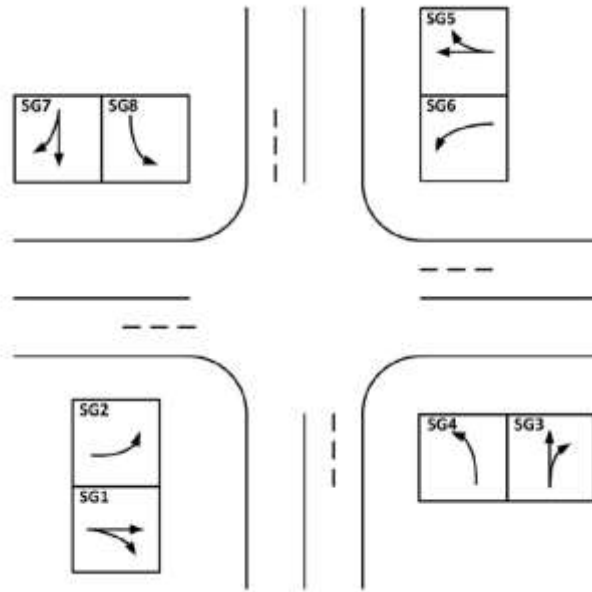
Figure 3.2. A group-based signal control scheme (Jin & Ma, 2017).
