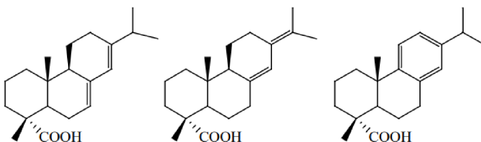
Abietic acid
