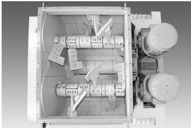
Figure 7: Twin-Shaft Mixer [23]
