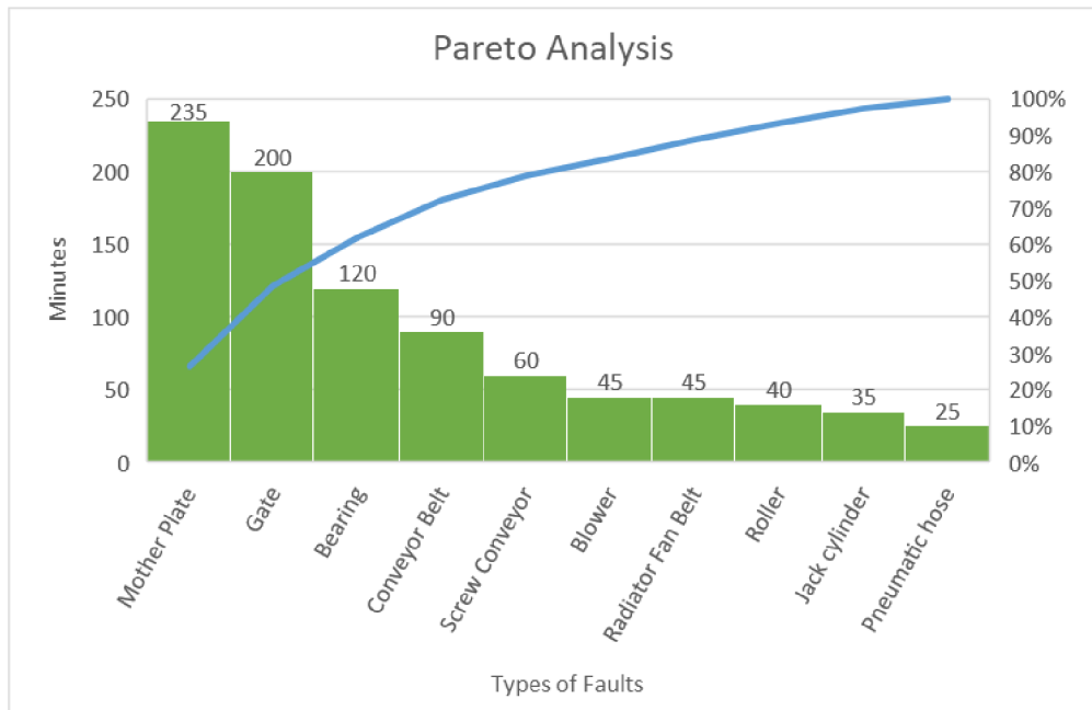
Graph 1: Pareto Analysis [20]
