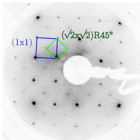
Figure 4.7: LEED pattern of the clean Fe 3 O 4 (001) surface after exposure to inert gas and liquid water. The reconstruction spots are visible, but very weak.
