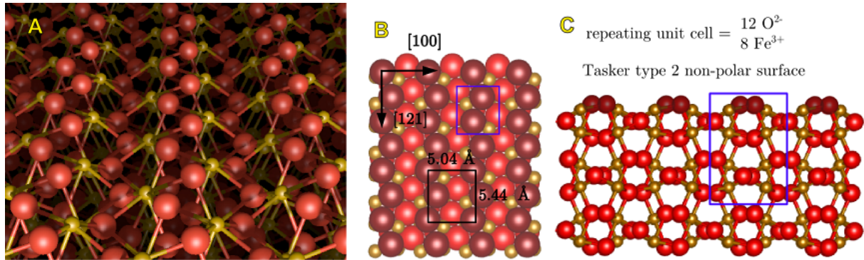
Figure 4.14: Bulk terminated hematite (012) surface. A) Perspective view on the bulk terminated hematite (012) (1 × 1) reconstructed surface. Oxygen atoms are red, iron atoms are yellow. B) Space-filling top view on the bulk terminated (1 × 1) surface. The surface oxygens are highlighted by dark red colour. C) Ball-and-stick side view on the bulk terminated (1 × 1) surface. The surface oxygens are highlighted by dark red colour. The repeating unit cell is highlighted by blue rectangle in pictures B and C. The cell has zero dipole moment, therefore the surface is classified as Tasker type 2 non polar.
