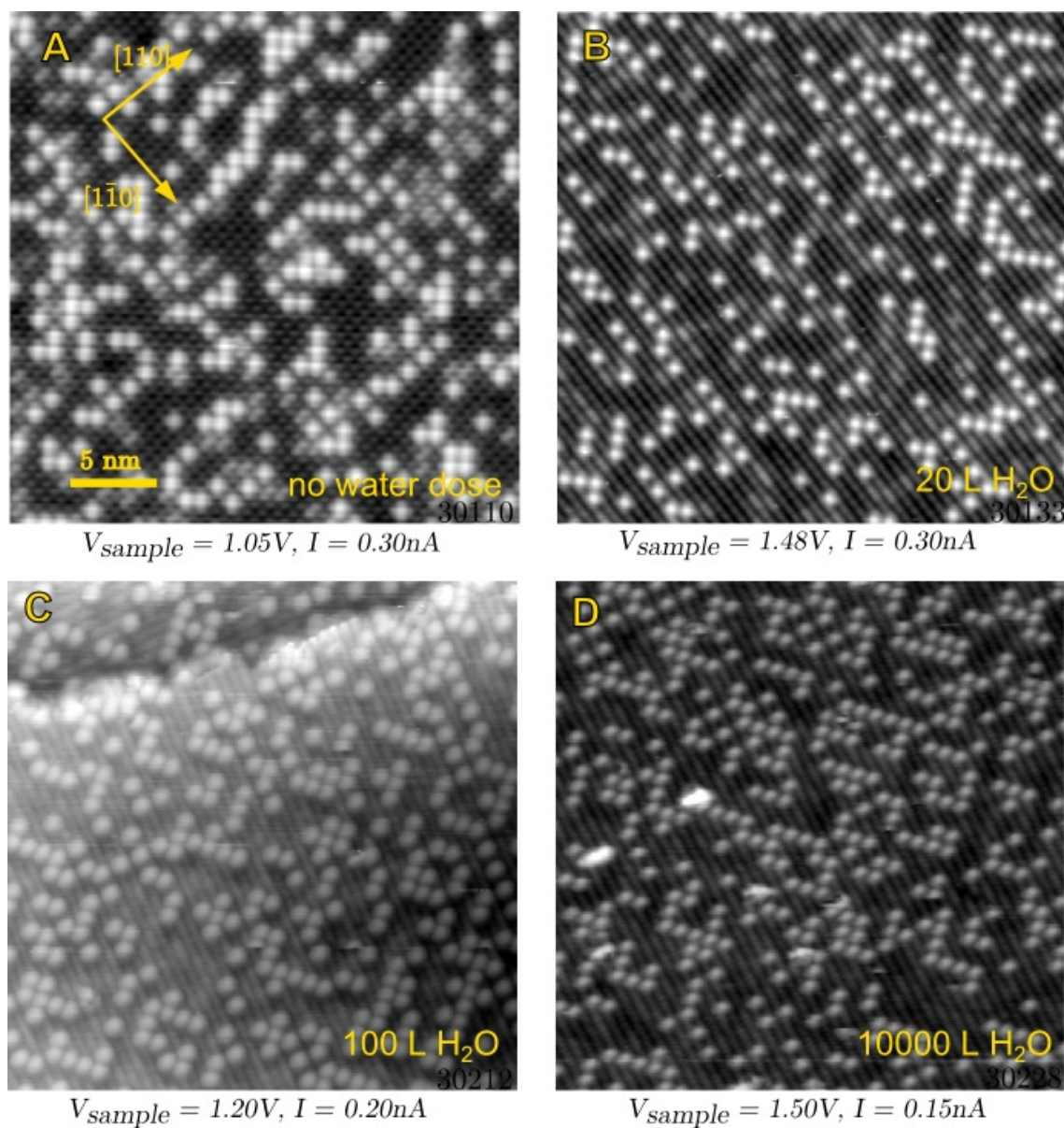
Figure 4.9: STM images of Ag adatoms (coverage 0.25 \pm 0.10 ML) on \text{Fe}_3\text{O}_4(001) surface after dosing \text{H}_2\text{O} . A) before dosing, B) dosed 20 L \text{H}_2\text{O} , C) dosed 100 L \text{H}_2\text{O} , D) dosed 10000 L \text{H}_2\text{O} .
