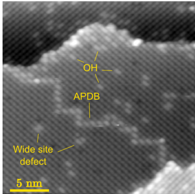
Figure 4.1: Typical STM image ( V_{\text{sample}} = 1.2 V, I = 0.2 nA) of the \text{Fe}_3\text{O}_4(001) surface after preparation. The undulating rows are oriented perpendicular to the rows on neighboring terraces. The characteristic defects (surface hydroxyls, anti-phase domain boundary and stationary wide site defects) are labeled.
