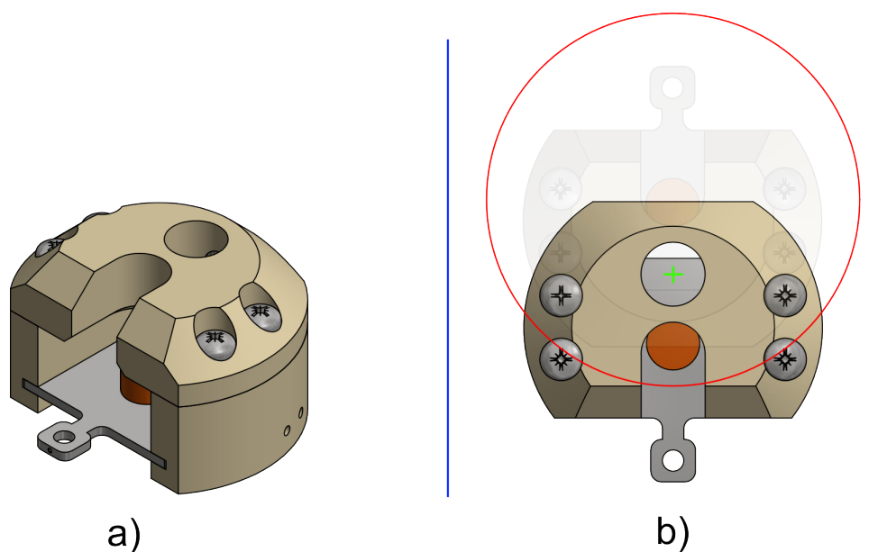
Figure 3.10: Sample holder made of PEEK. The sample plate can be inserted facing both up or down while being in reach of the drop maker. In picture b) the off-centre design is highlighted. Axis of rotation is the green cross. The blue lines indicate the inner tube of the glass jar (diameter 42 mm), the red circle is inner diameter of both NS ground joints used for the vertical transfer (35 mm). It can be seen, that the place where the sliding metal-to-metal contact would take place is not directly above the cell (red circle is approx. 5 mm away from the ear). Then the whole PEEK holder is rotated and can be lowered through the NS ground joint (red circle) to the cell.
