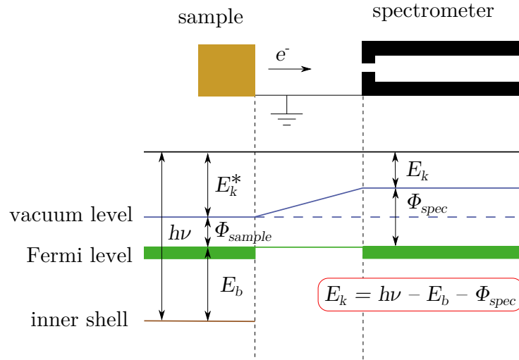
Figure 2.4: Illustration of equation 2.9. Picture adapted from [49]
