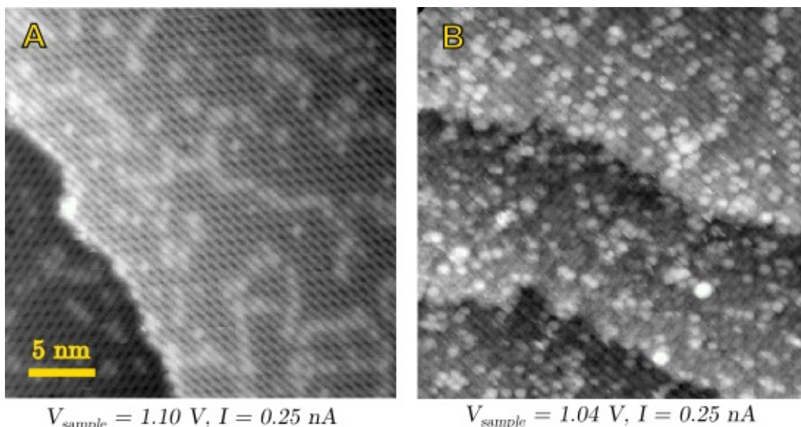
Figure 4.5: STM images of clean Fe 3 O 4 (001) before and after exposure to air and liquid water.
