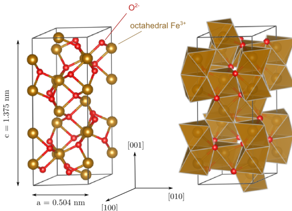
Figure 1.6: Ball-and-stick and polyhedral models of hematite unit cell. The oxygen forms slightly distorted hcp lattice. Two thirds of the octahedral sites are filled with iron, which can be seen on the polyhedral model - in the [001] direction there are always two face-sharing octahedra followed by one missing. Note the coordinate system is trigonal, not cartesian.
