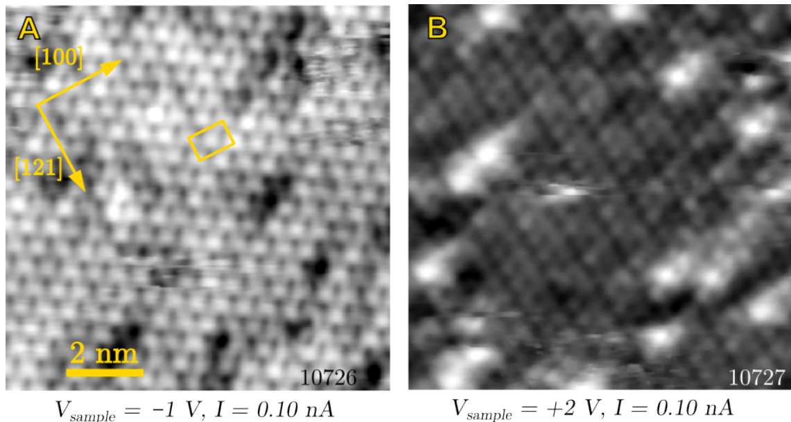
Figure 4.15: Filled states (left) and empty states (right) STM images of the (2 × 1) reconstructed surface of hematite (012). The (2 × 1) unit cell is highlighted by the yellow rectangle.
