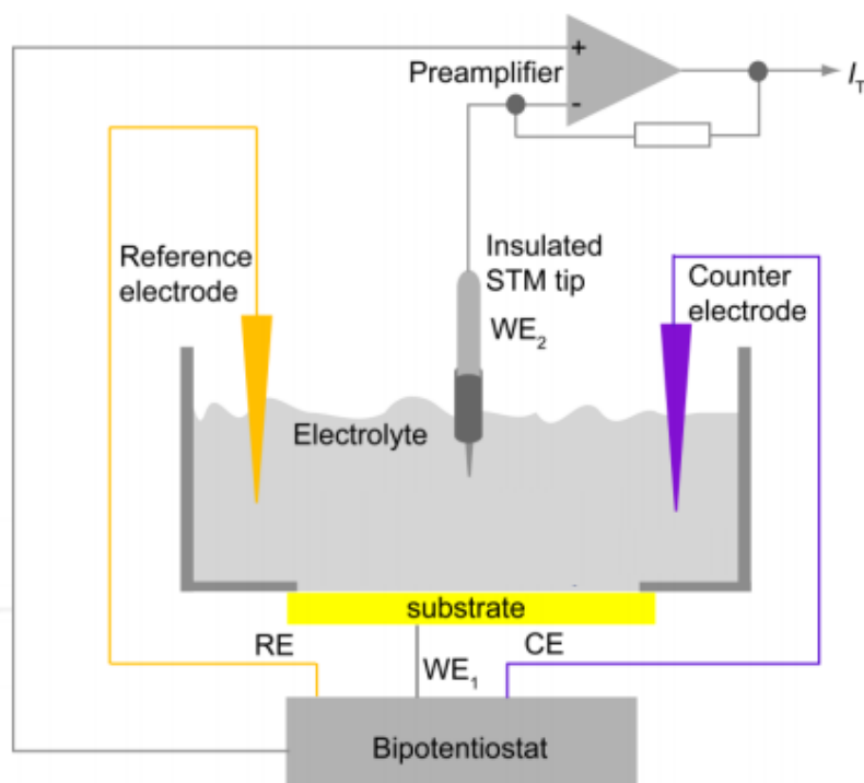
Figure 2.13: Setup of in-situ EC-STM, picture adapted from [53]
