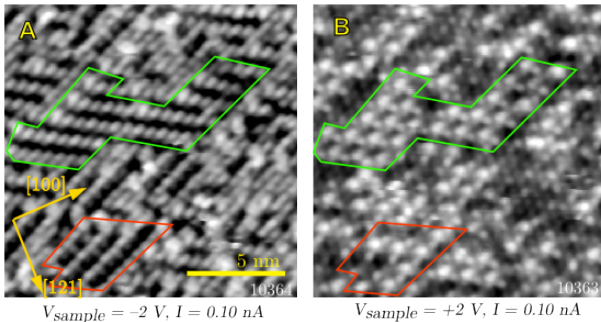
Figure 4.19: Filled (A) and empty (B) states image of the same spot on the patched reconstruction of the hematite (012) ( 2 \times 1 ) reconstructed surface. The 1D chains can be seen in both images (as highlighted by the red and green lines), although in filled states they are much clearer. In empty states the repeating unit of the chain consists of two different species with one of them much more pronounced. In filled states, the chains look homogeneous.
