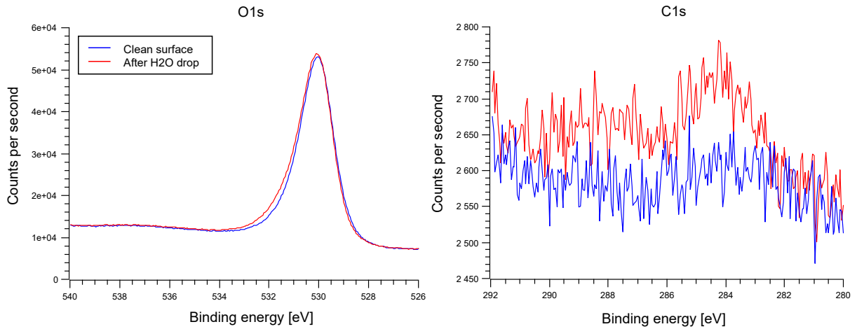
Figure 4.6: XPS analysis of the surface before and after exposure to air and liquid H 2 O. The shoulder on the O1s peak indicates hydroxylation of the surface. The C1s peak, almost non-existent on the clean surface, is much higher on the surface after exposure to air and water.
