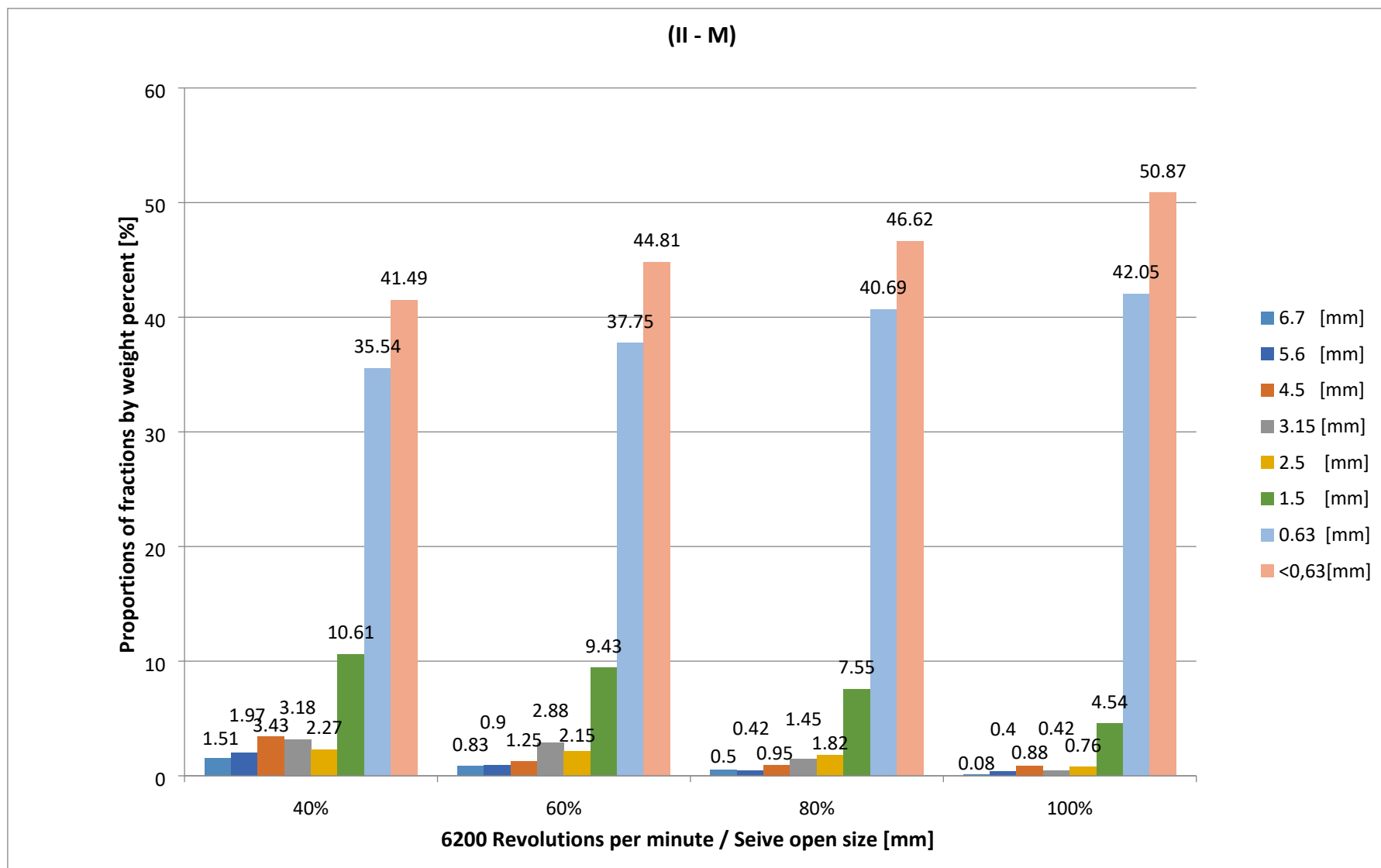
Figure 40. Particle size distribution according to rotor speed for (II – M) [mm]
