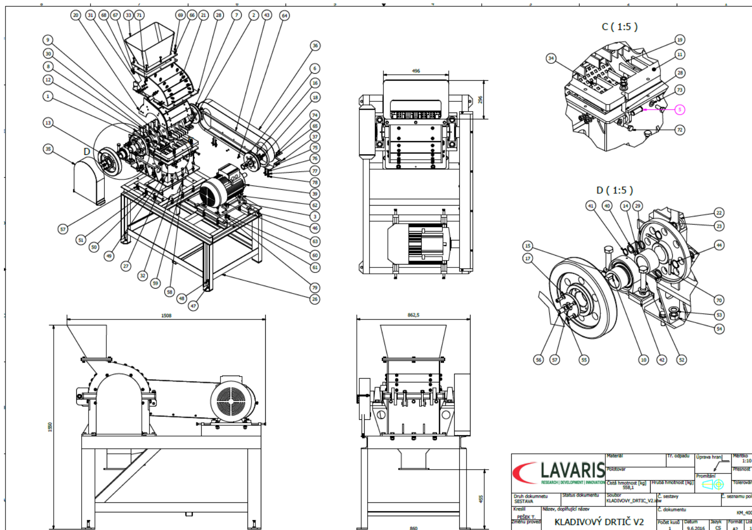
Figure 4. Hammer mill LAV/ HM-350. Source: LAVARIS
