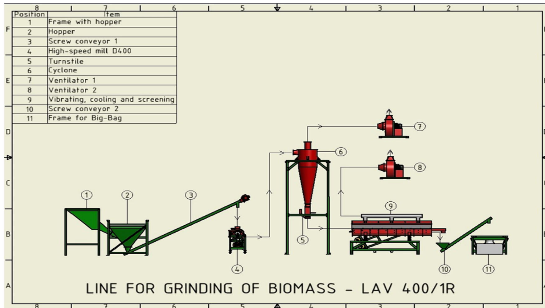
Figure 11. Scheme of the Line for grinding and drying of Biomass
