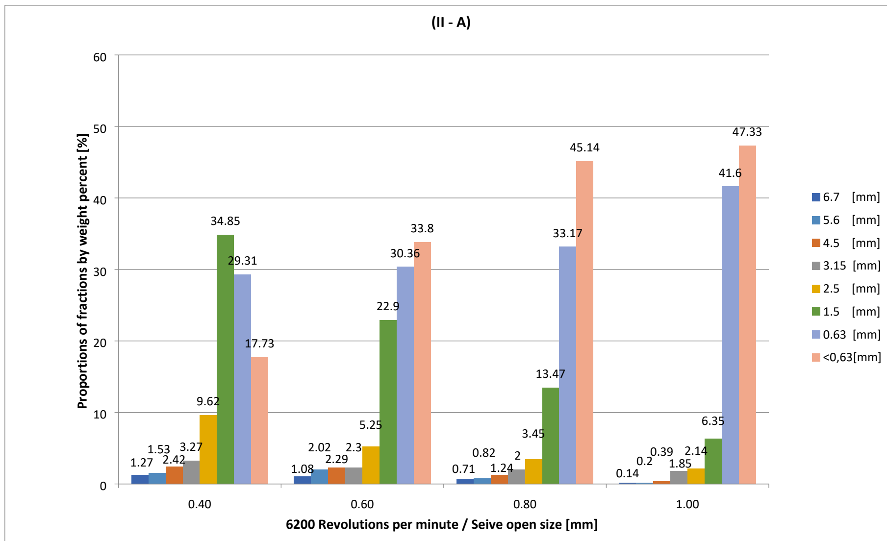
Figure 32. Particle size distribution according to rotor speed for (II – A) [mm]
