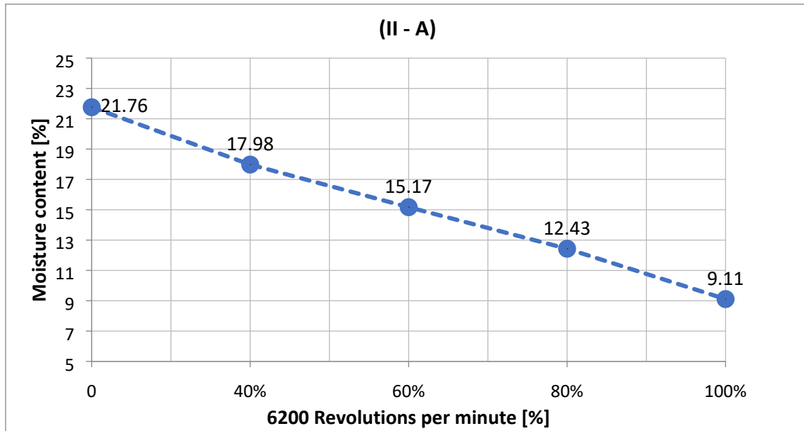
Figure 33. Moisture content related to rotors speed for (II – A)
