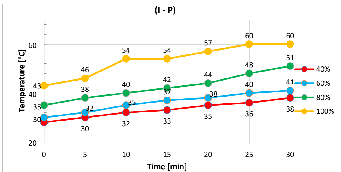
Figure 43. Temperature related to time for (I – P)
