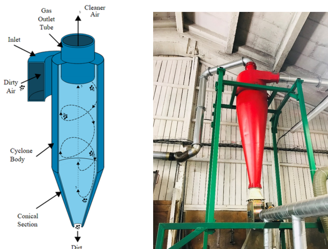
Figure 18. Cyclone with rotary feeder
