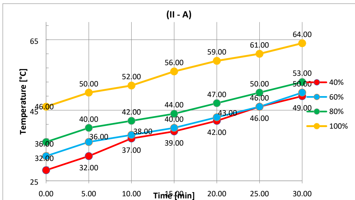
Figure 31. Temperature related to time for (II – A)
