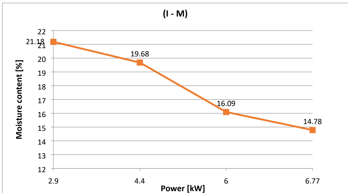
Figure 38. Power related to moisture content for (I – M)
