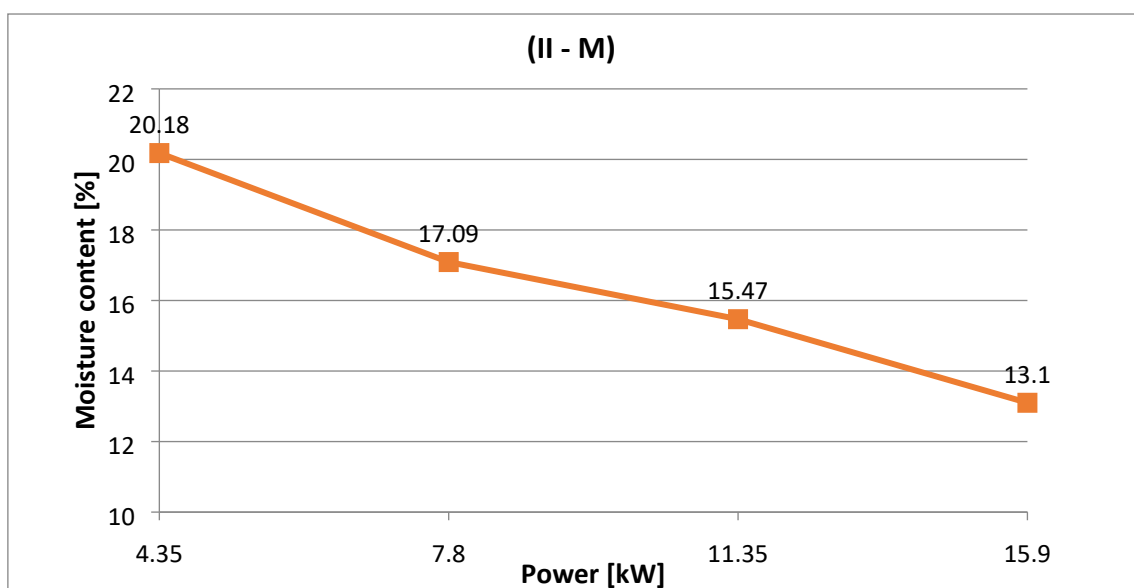
Figure 42. Power related to moisture content for (II – M)
