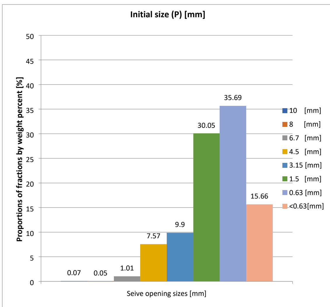
Figure 10. Initial particle size distribution for Pine sawdust wood
