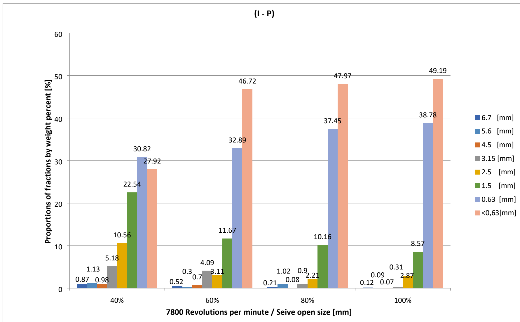
Figure 44. Particle size distribution according to rotor speed for (I – P) [mm]
