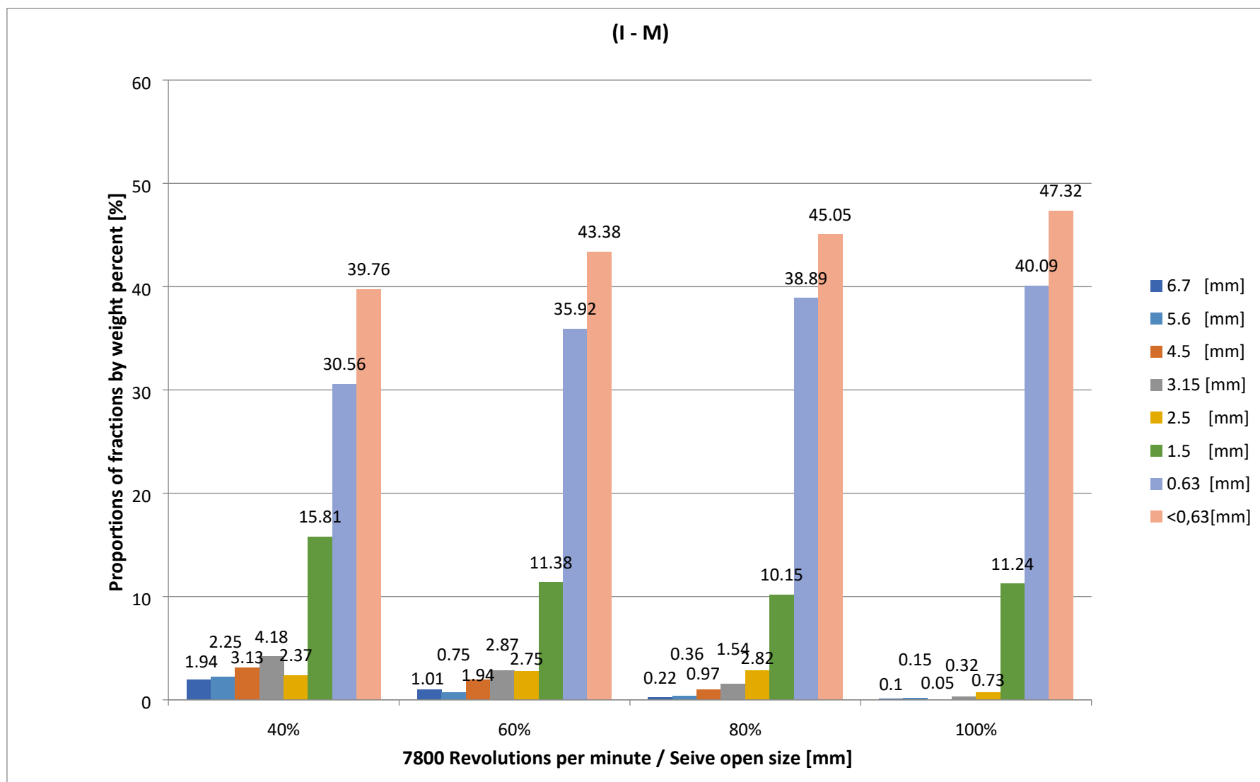
Figure 36. Particle size distribution according to rotor speed for (I – M) [mm]
