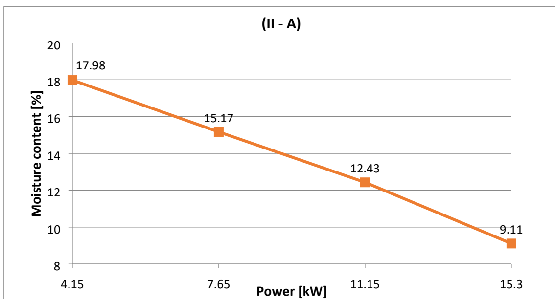
Figure 34. Power related to moisture content for (II – A)
