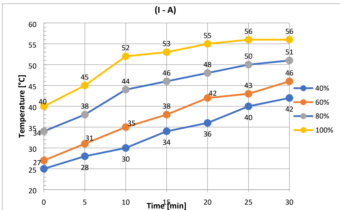
Figure 27. Temperature related to time for (I – A)
