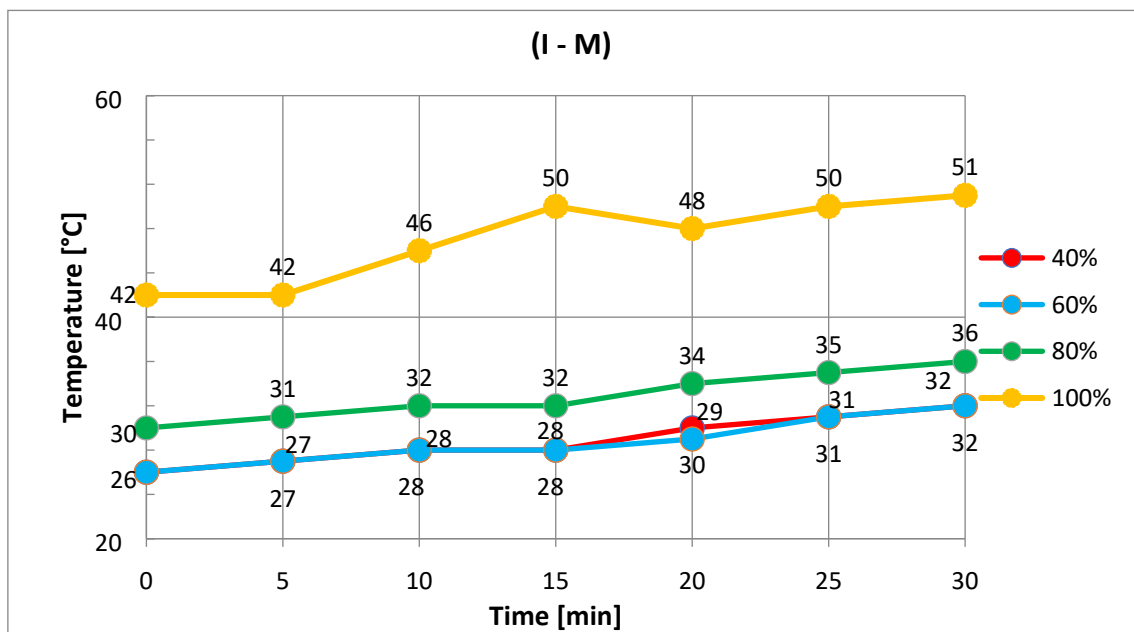
Figure 35. Temperature related to time for (I – M)
