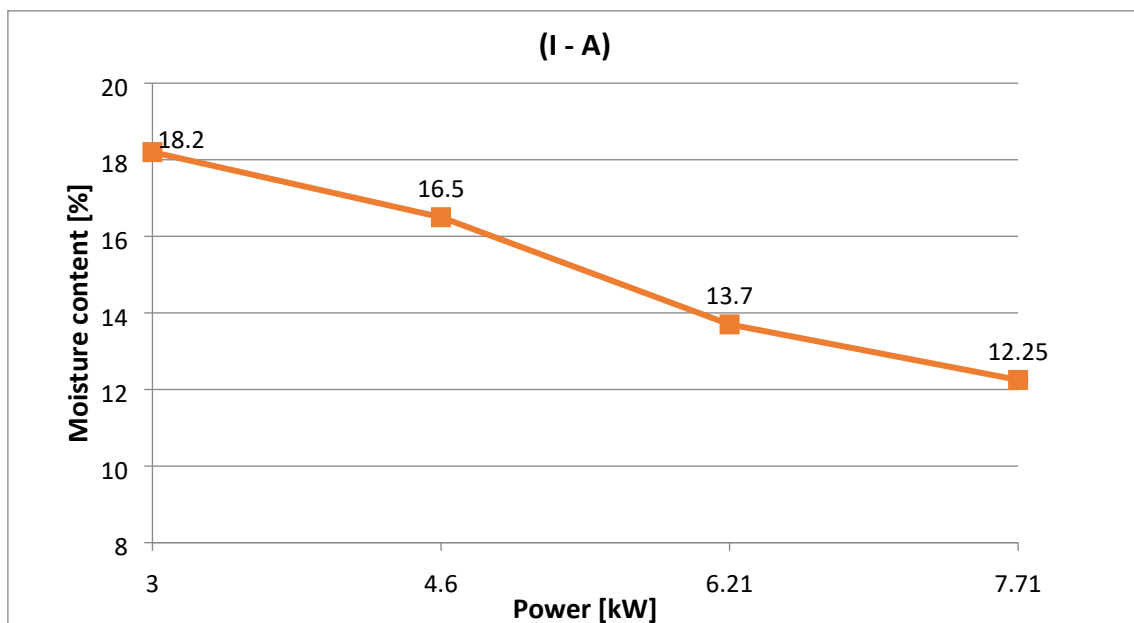
Figure 30. Power related to moisture content (I - A)
