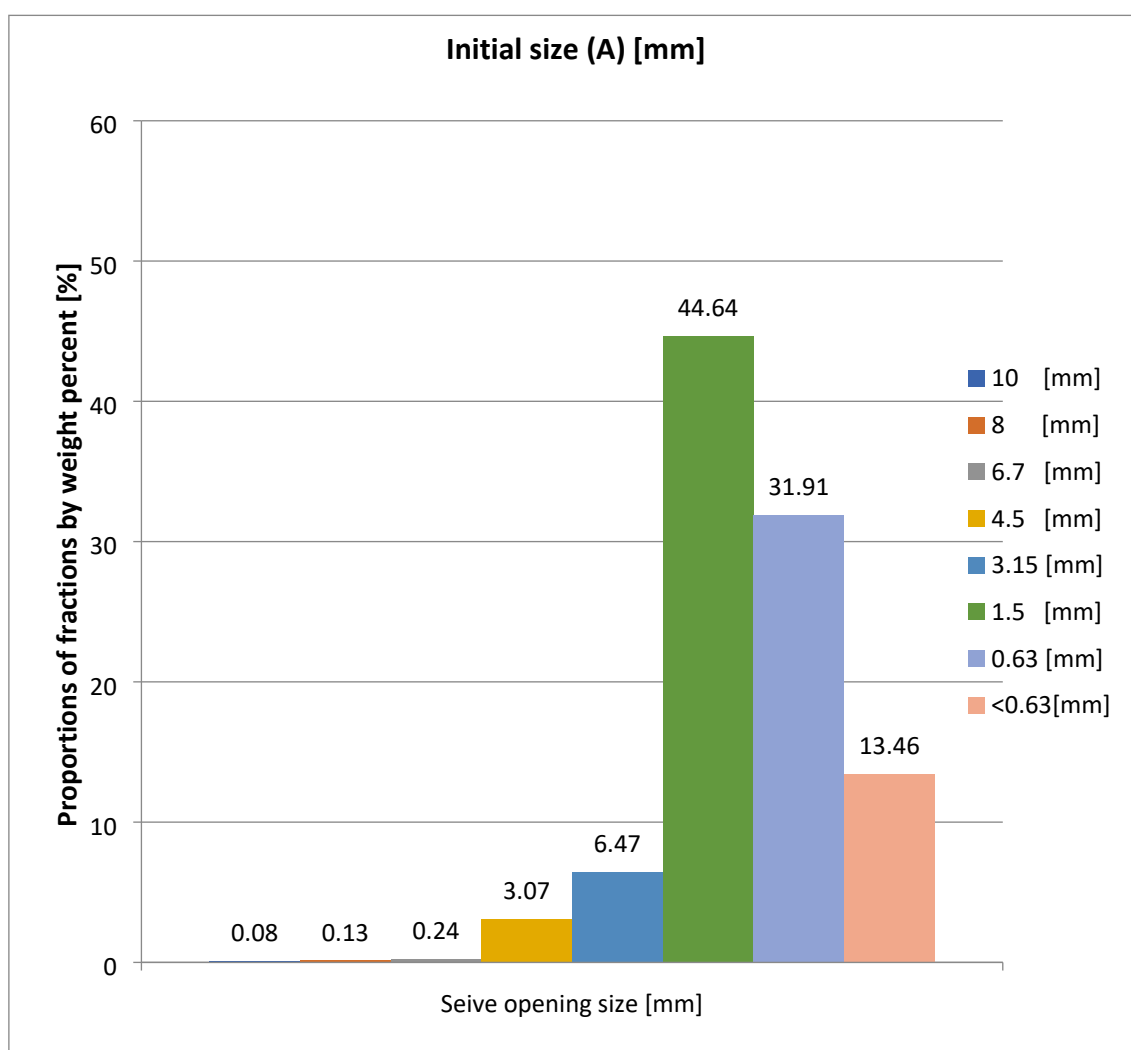
Figure 8. Initial particle size distribution for Apple tree wood
