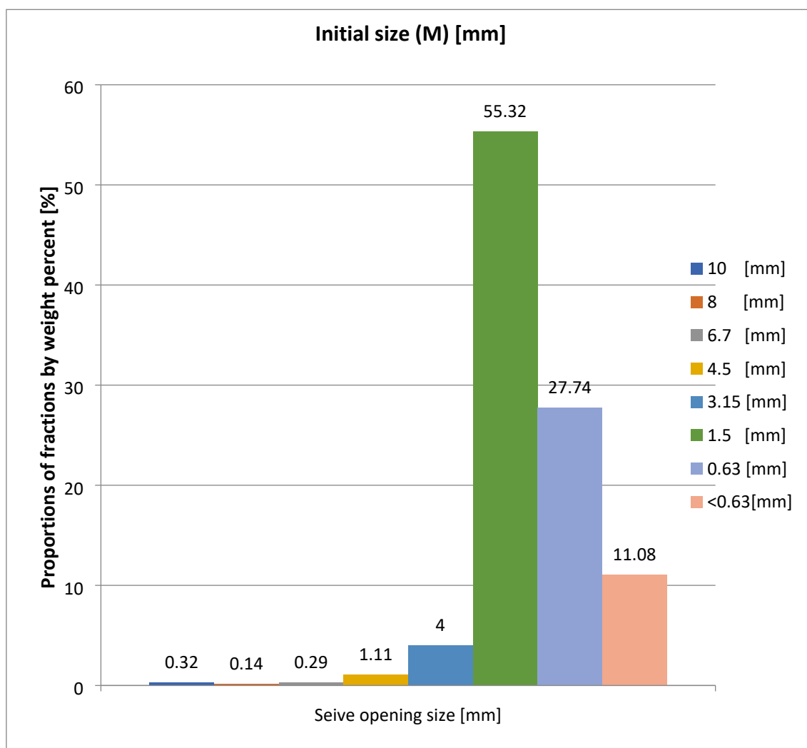
Figure 9. Initial particle size distribution for Miscanthus sinensis
