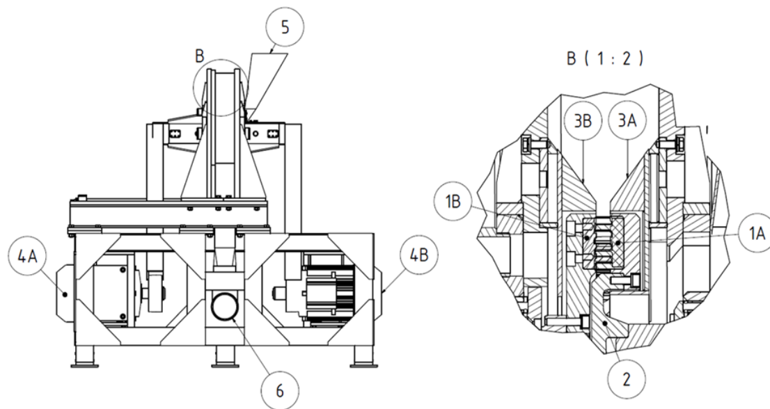
Figure 16. Detailed technical drawings of LAV 300/2R
