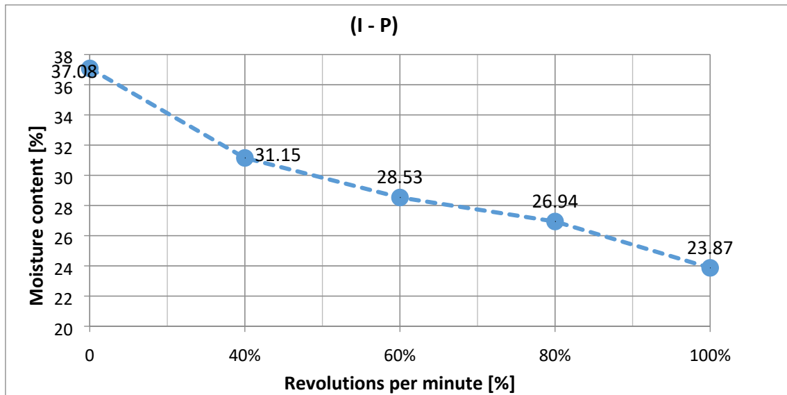
Figure 45. Moisture content related to rotor speed for (I - P)
