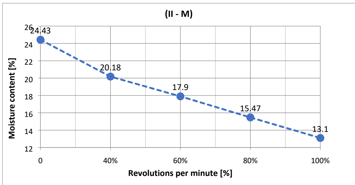
Figure 41. Moisture content related to Rotor speed for (II – M)
