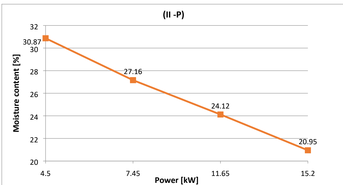
Figure 50. Power related to moisture content for (II - P)
