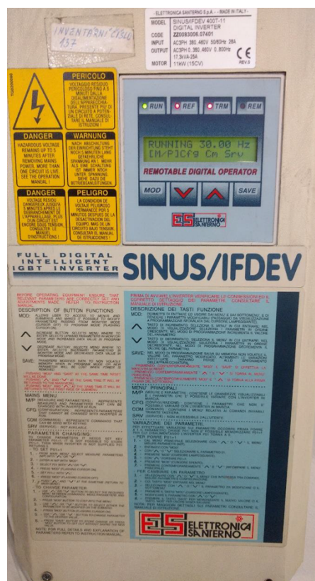
Figure 21. Ventilator frequency inverter
