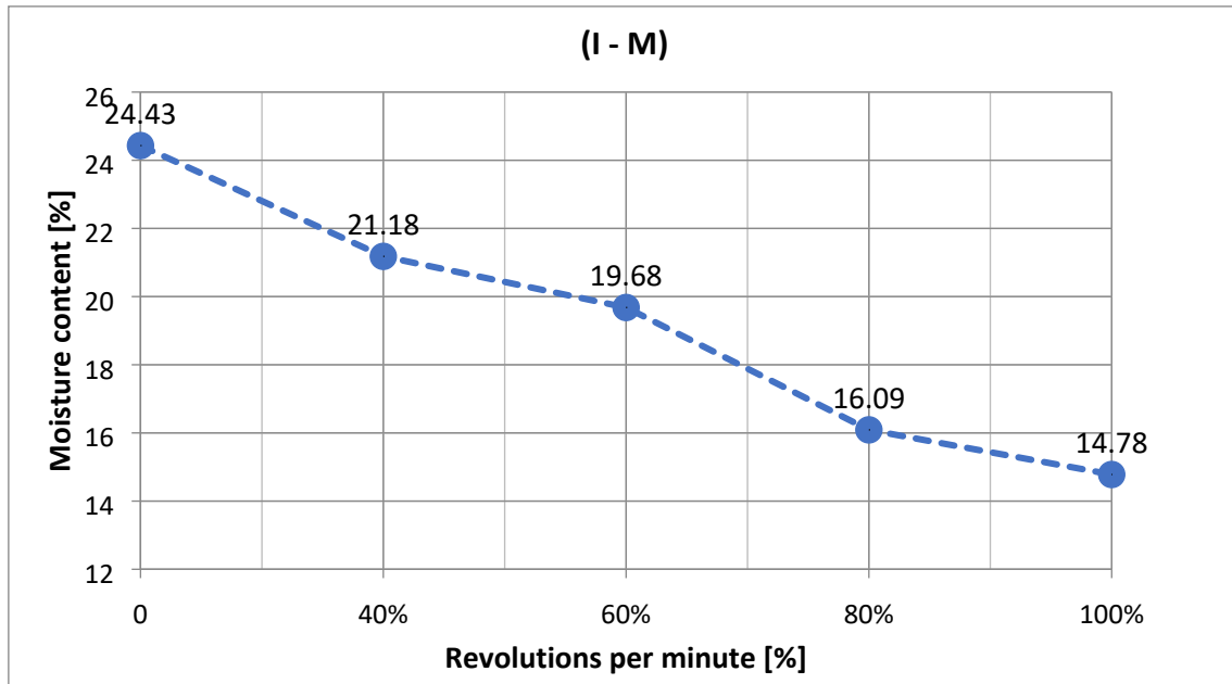
Figure 37. Moisture content related to Rotor speed for (I – M)
