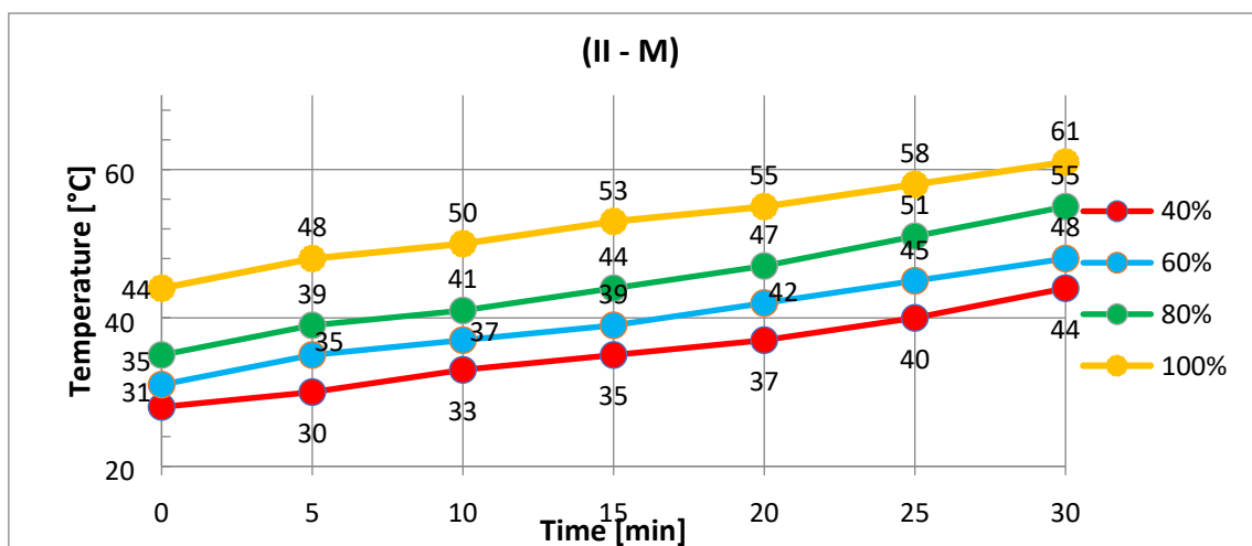
Figure 39. Temperature related to time for (II – M)
