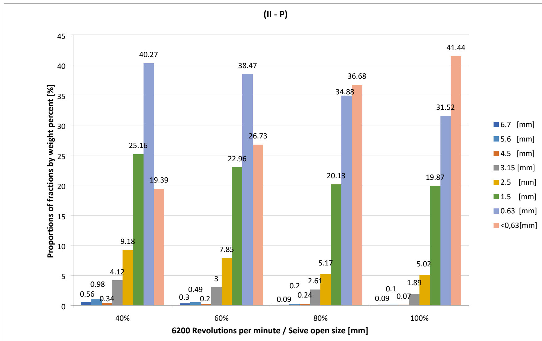
Figure 48. Particle sizes distribution related to rotor speed for (II – P) [mm]
