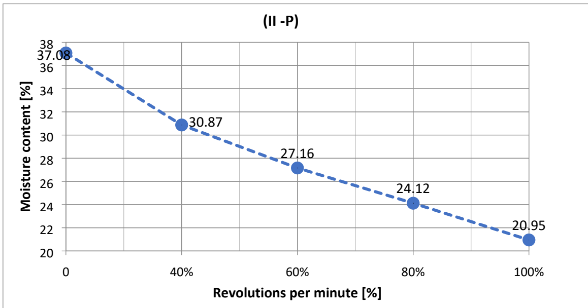
Figure 49. Moisture content related to rotor speed for (II - P)
