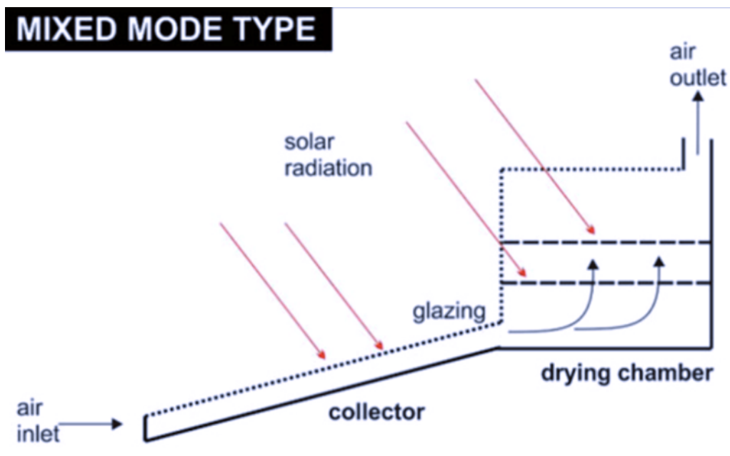
Figure 5. Mixed mode dryer. Source: Prakash et al. (2017)
