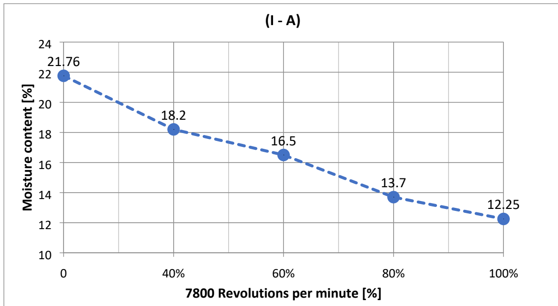
Figure 29. Moisture content related to rotor speed for (I – A)
