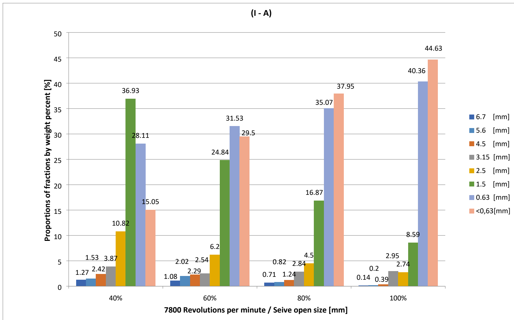
Figure 28. Particle size distribution according to rotor speed for (I – A) [mm]
