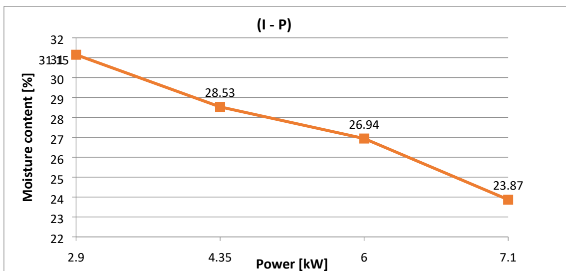
Figure 46. Power related to moisture content for (I - P)
