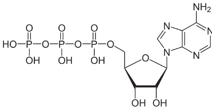
Figure 3: Chemical structure of adenosine triphosphate (Vang, 2013)
