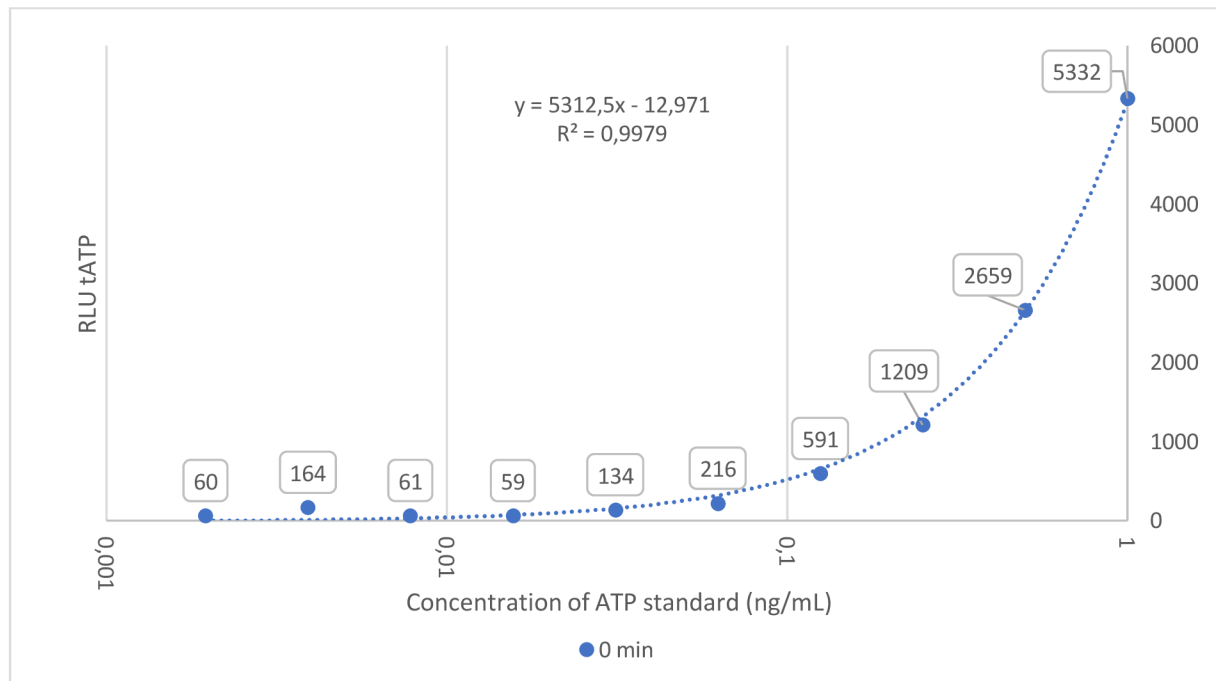
Figure 6: Standardisation curve for the DeltaTox kit
