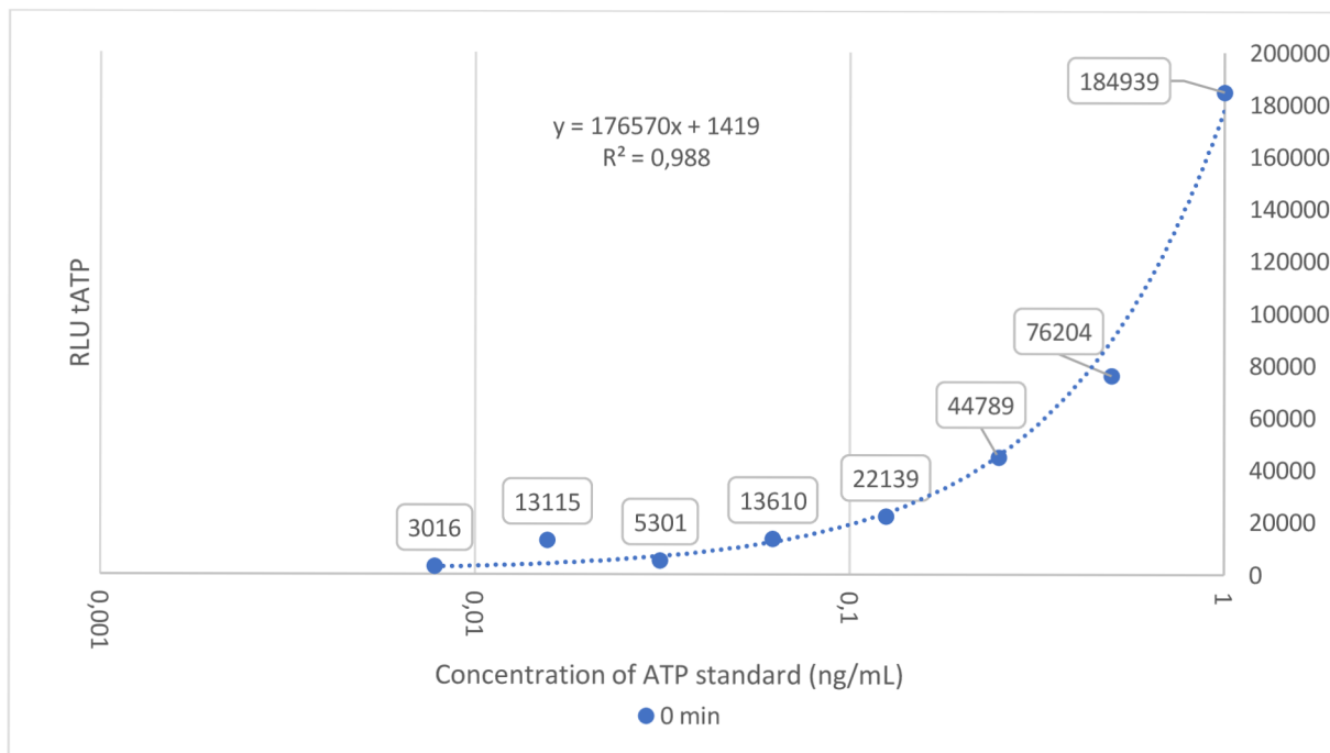
Figure 7: Standardization curve for the FLAA ATP standard
