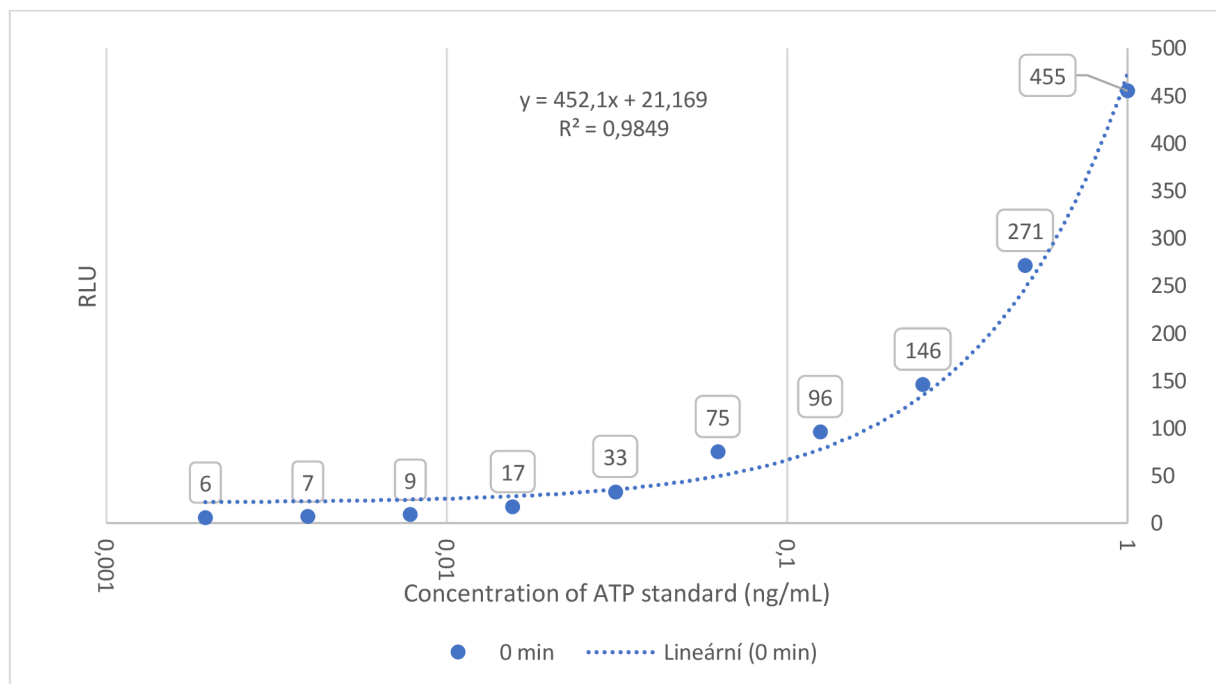
Figure 9: Standardization curve for the SystemSURE Plus kit
