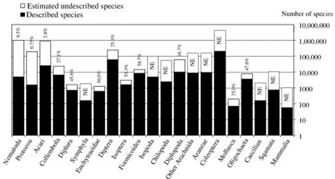
Figure 1: Estimated numbers of described and un-described species for major soil animal taxa (Decaëns et al. 2006), NE = no estimation available.
