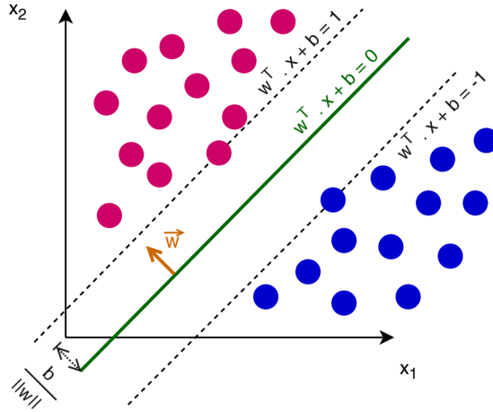
Figure 3.3: SVM maximum-margin hyperplane.
