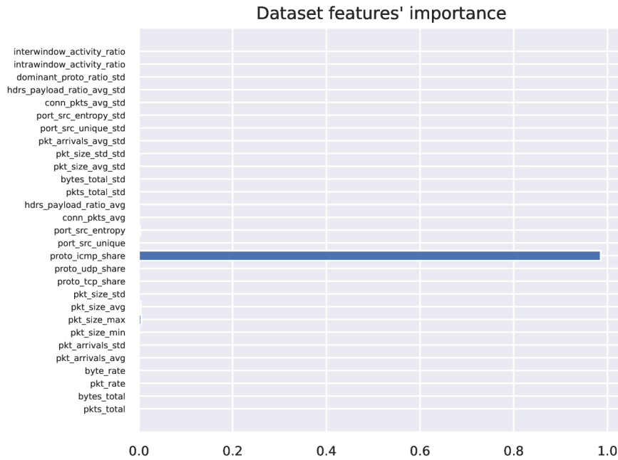
Figure 6.7: Decision Tree Gini features' importance for real dataset.
