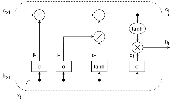
Figure 3.11: Long-Short Term Memory cell structure.
