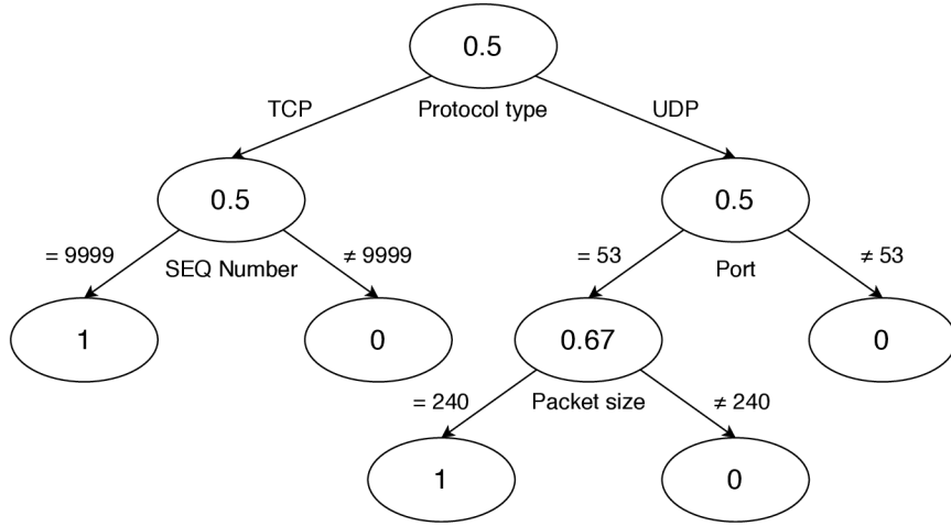
Figure 3.4: Decision tree based on Table 3.1 example.
