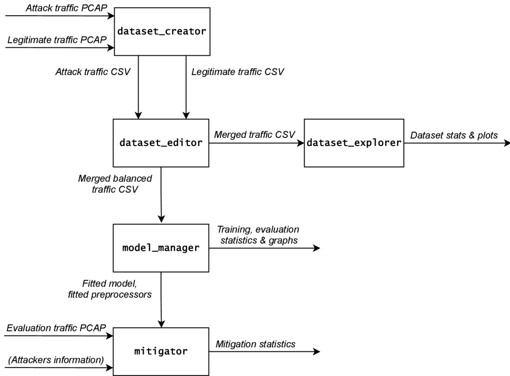
Figure 5.2: Implementation of the system pipeline through scripts.
