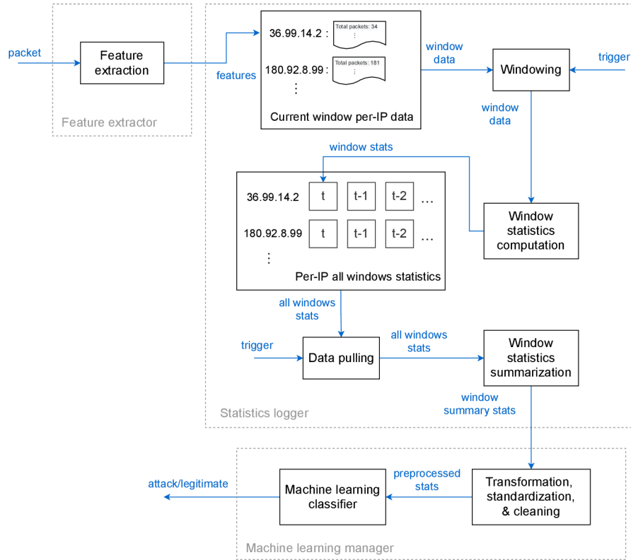
Figure 4.2: Detailed machine learning pipeline of the DDoS detection system.
