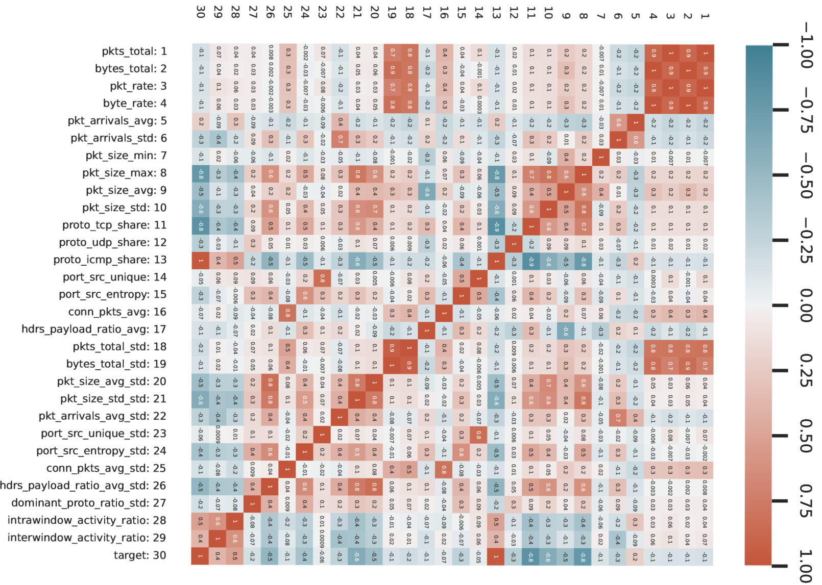
Figure 6.4: Real dataset features correlation.
