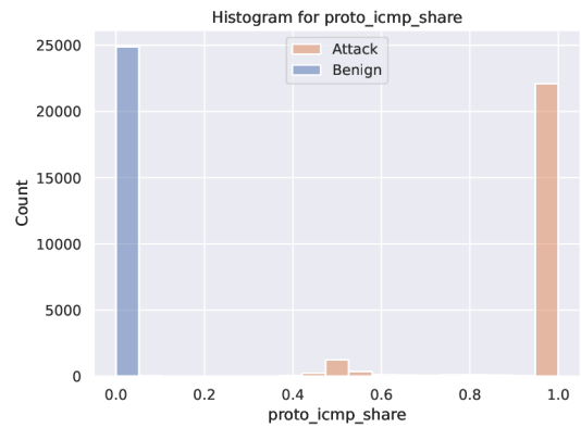
(b) ICMP Protocol share.
