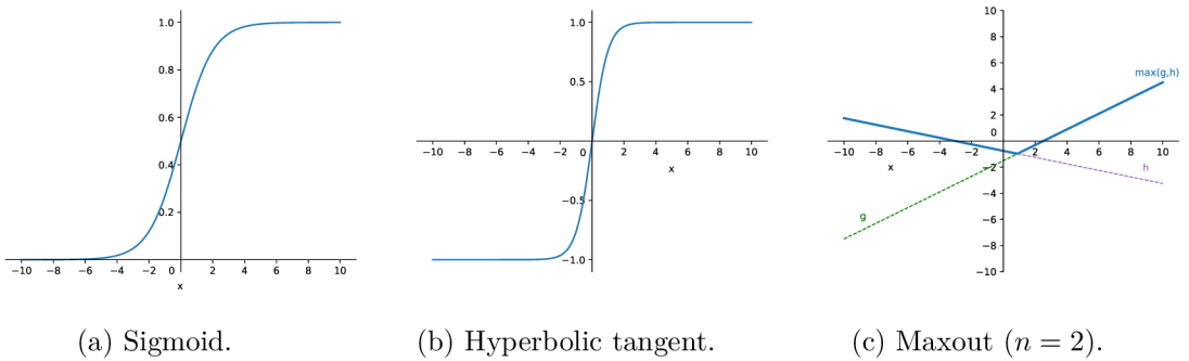
Figure 3.7: Examples of various activation functions.
