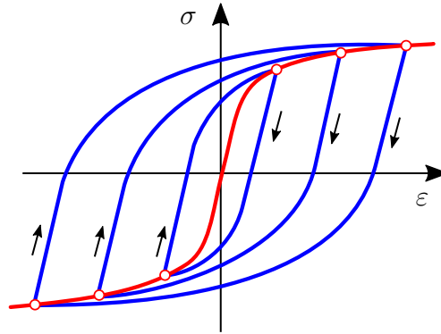
Figure 3.6: An example of cyclic stress–strain curve, depicted by the red line [25]
