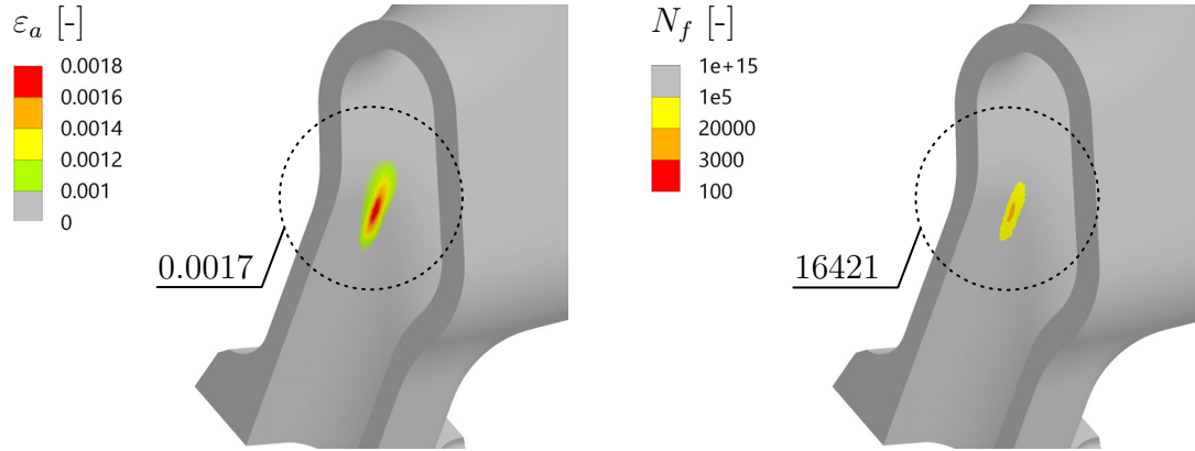
Figure 4.47: \varepsilon_a and N_f predicted using the strain-based approach, BKIN material model
