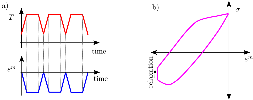
Figure 3.14: Example of OPTMF with dwell periods, a) control quantities, b) stress response, re-created from [60]
