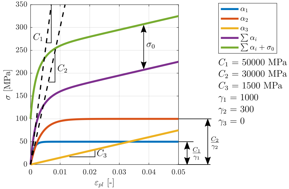
Figure 2.8: Decomposition of Chaboche model for k = 3 for illustration purposes, inspired by [35, 36]
