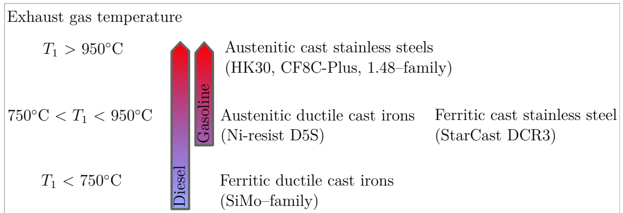
Figure 3.2: Approximate division of the material groups used in hot end components, with respect to exhaust gas temperature [42, 62]
