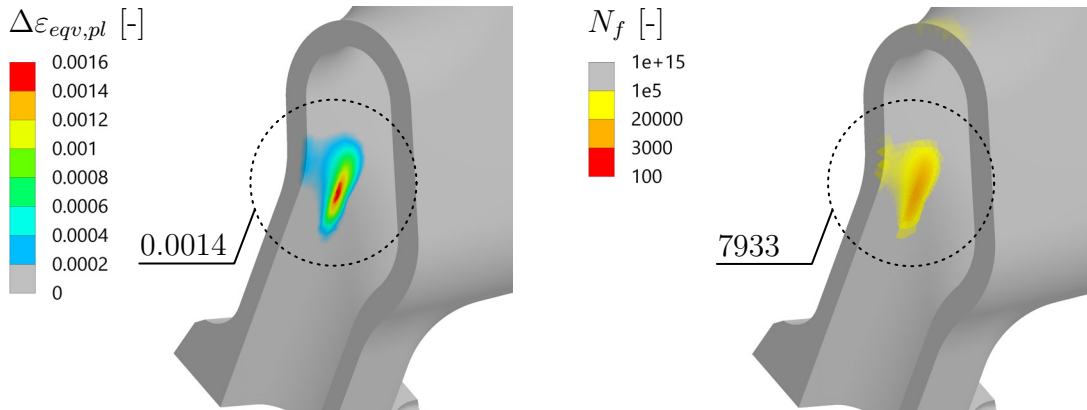
Figure 4.46: \Delta\varepsilon_{eqv,pl} and N_f predicted using an energy-based approach on a refined mesh, BKIN material model
