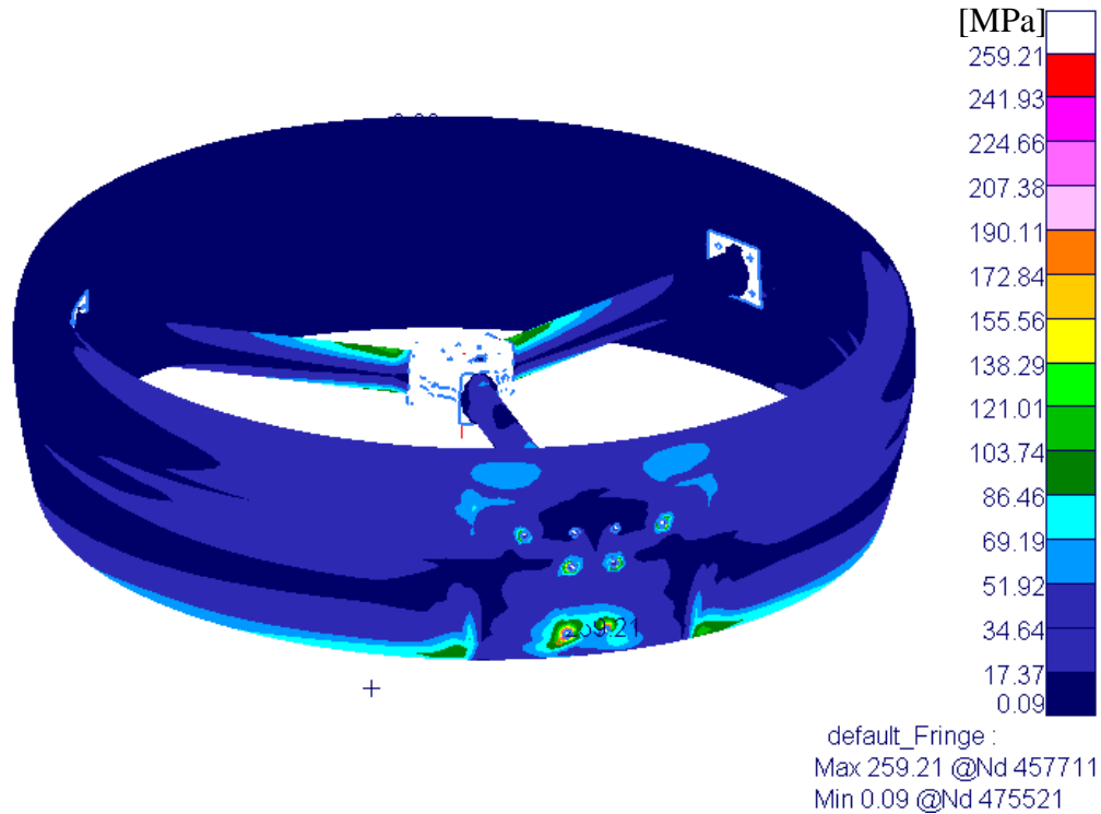
Figure 10.14 Shear stress distribution on composite parts
