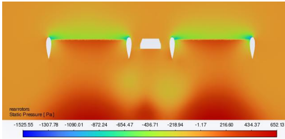
Figure 11.13 Static pressure [Pa] of rear rotors at 0.5 m above ground
