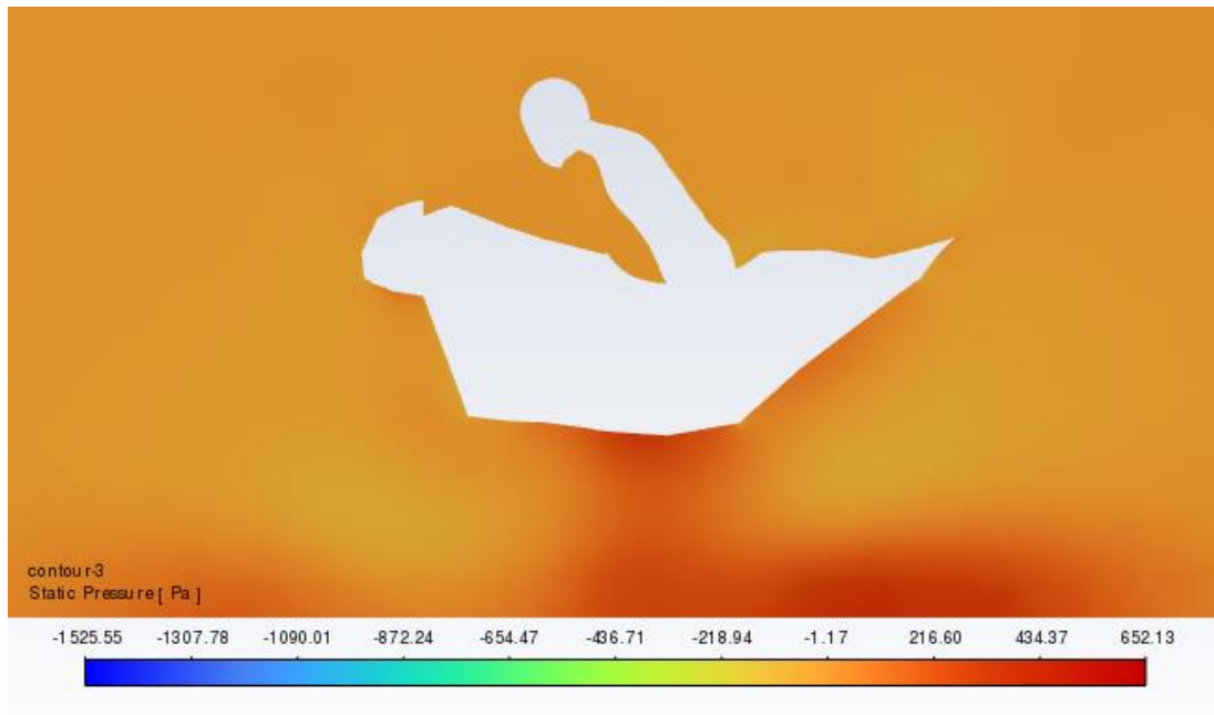
Figure 17.2 Static pressure distribution at 0.5 m above ground (symmetry plane)
