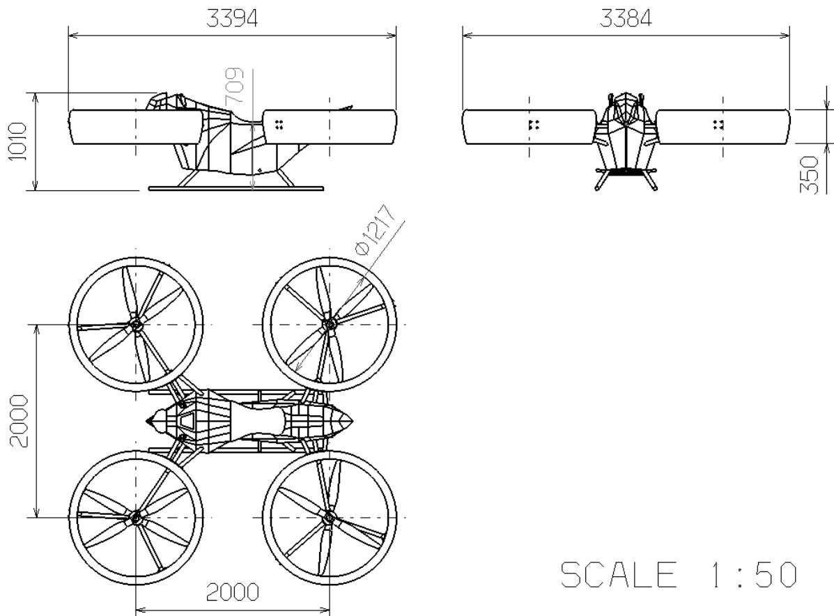
Figure 8.1 Drawing of final design
