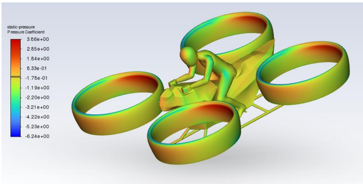
Figure 11.24 Pressure coefficient distribution on multicopter at 20° pitch angle
