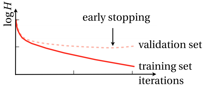
Figure 3.14: Progress of training and validation losses. The plot is schematic, and the data is smoothed. The training is stopped when the validation energy begins to increase. [3]
