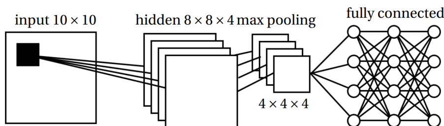
Figure 3.17: Schematic of the standard CNN topology for image classification. [3]
