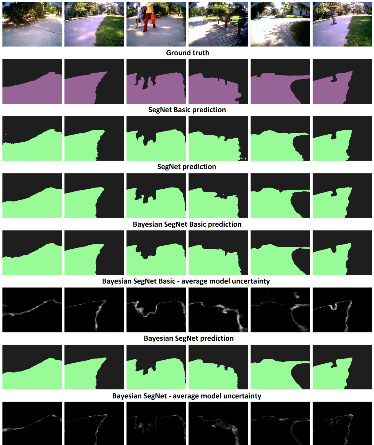
Figure 5.3: Comparison of the segmentation performance of all SegNet variants. The Bayesian versions of the architecture give the estimate of the model uncertainty, where the lighter regions mean higher variance across the MCDO samples taken during inference.
