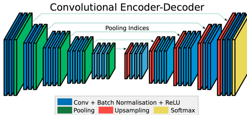
Figure 3.18: SegNet - an example of encoder-decoder CNN architecture. [25]
