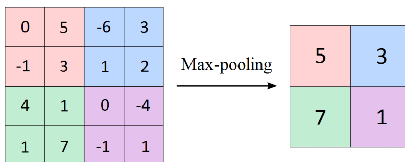
Figure 3.16: Max-pooling of size 2x2 and stride 2. [13]
