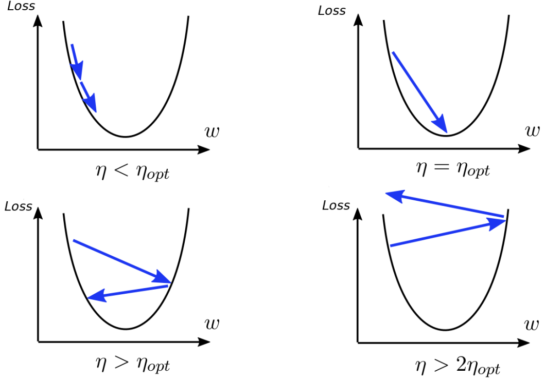
Figure 3.10: Effect of the learning rate on optimization: the value must be chosen carefully for the algorithm to converge. [13]
