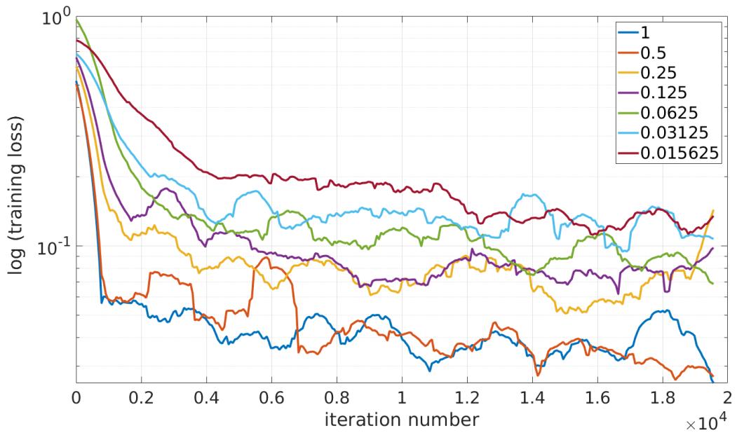
Figure 5.2: Coarse search of the learning_rate parameter, Bayesian SegNet. The training loss is observed for 30 epochs and the data is smoothed. The encoder was initialized using pre-trained VGG16 model and the learning rate of the corresponding layers is decreased by the factor of 10 during the training.
