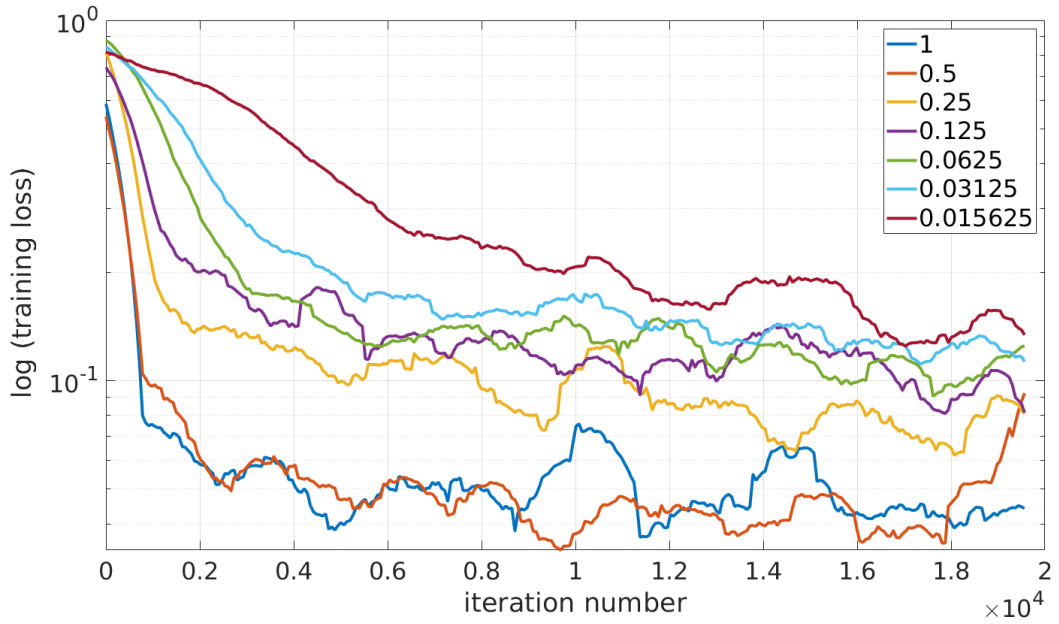
Figure 5.1: Coarse search of the learning_rate parameter, Bayesian SegNet. The training loss is observed for 30 epochs and the data is smoothed. The encoder was initialized using pre-trained VGG16 model and the corresponding layers stayed unchanged during the training.
