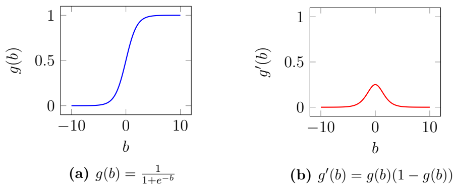
Figure 3.2: Sigmoid function and its derivative. Notice that the derivative goes to zero very quickly.
