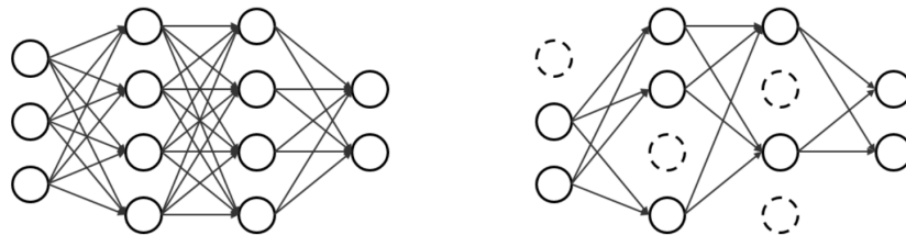
Figure 3.13: ANN without (left) and with dropout (right). [17]
