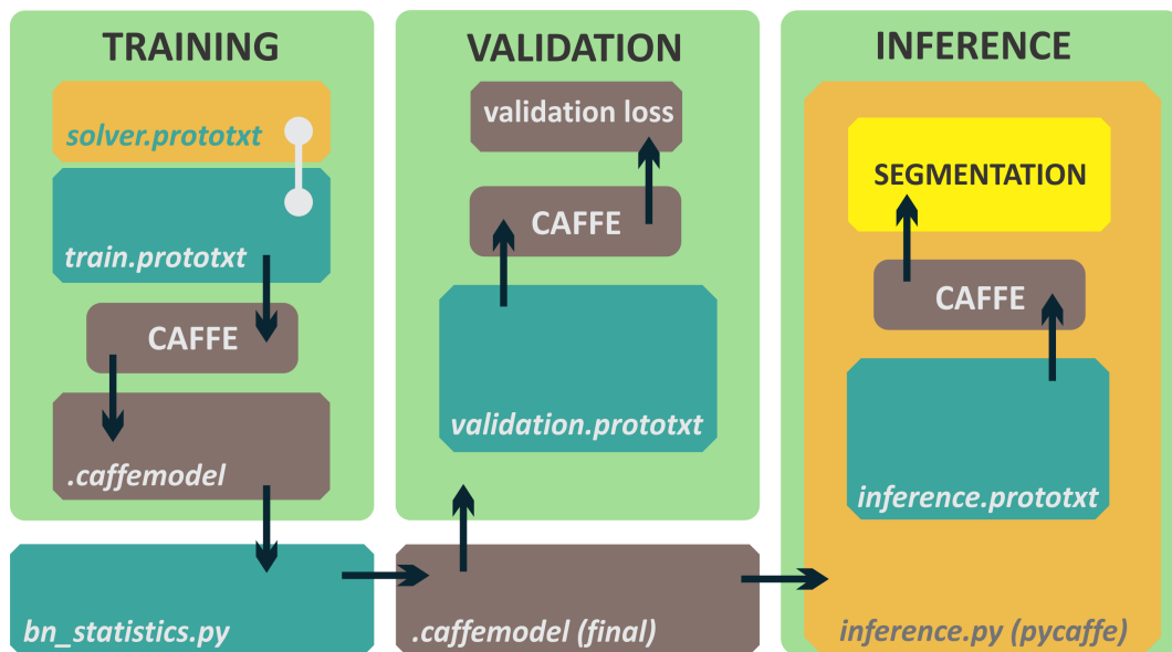
Figure 4.3: Using Caffe implementation of SegNet - schematic diagram.
