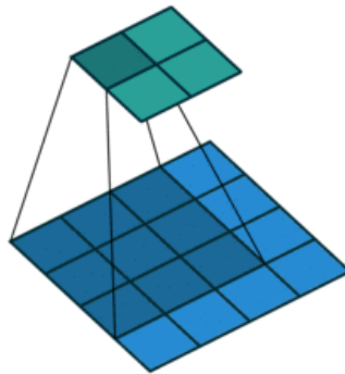
Figure 3.19: Transposed convolution. [37]
