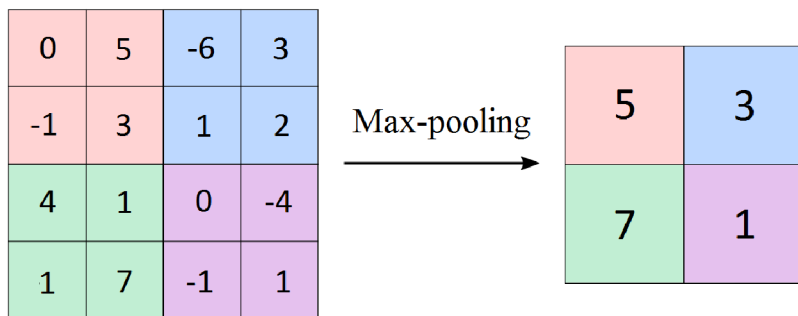
Figure 3.16: Max-pooling of size 2x2 and stride 2. [13]
