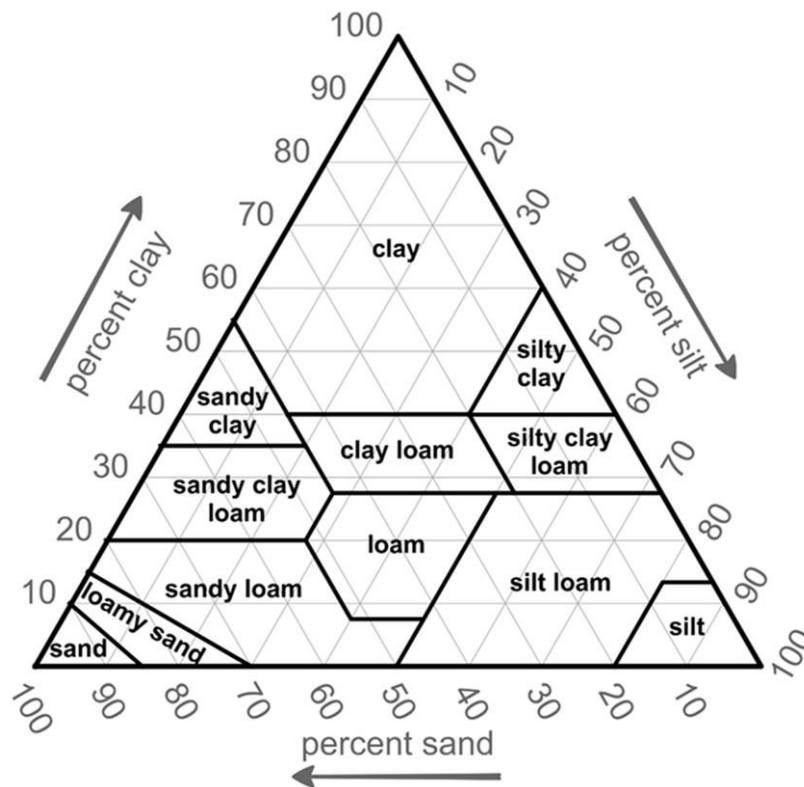
Fig.9. Soil texture triangle (Groenendyk et al. 2015).
