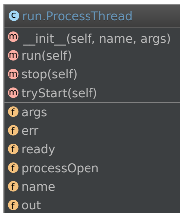
Obr. 5.1: Trieda processThread
