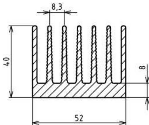
Obr. 13 – Chladič K52 [17]
