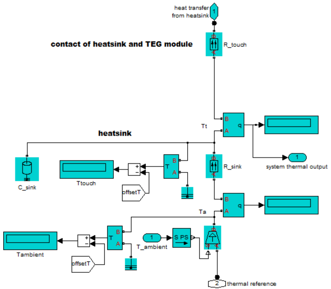
Obr. A7 – Subsystem HEATSINK
