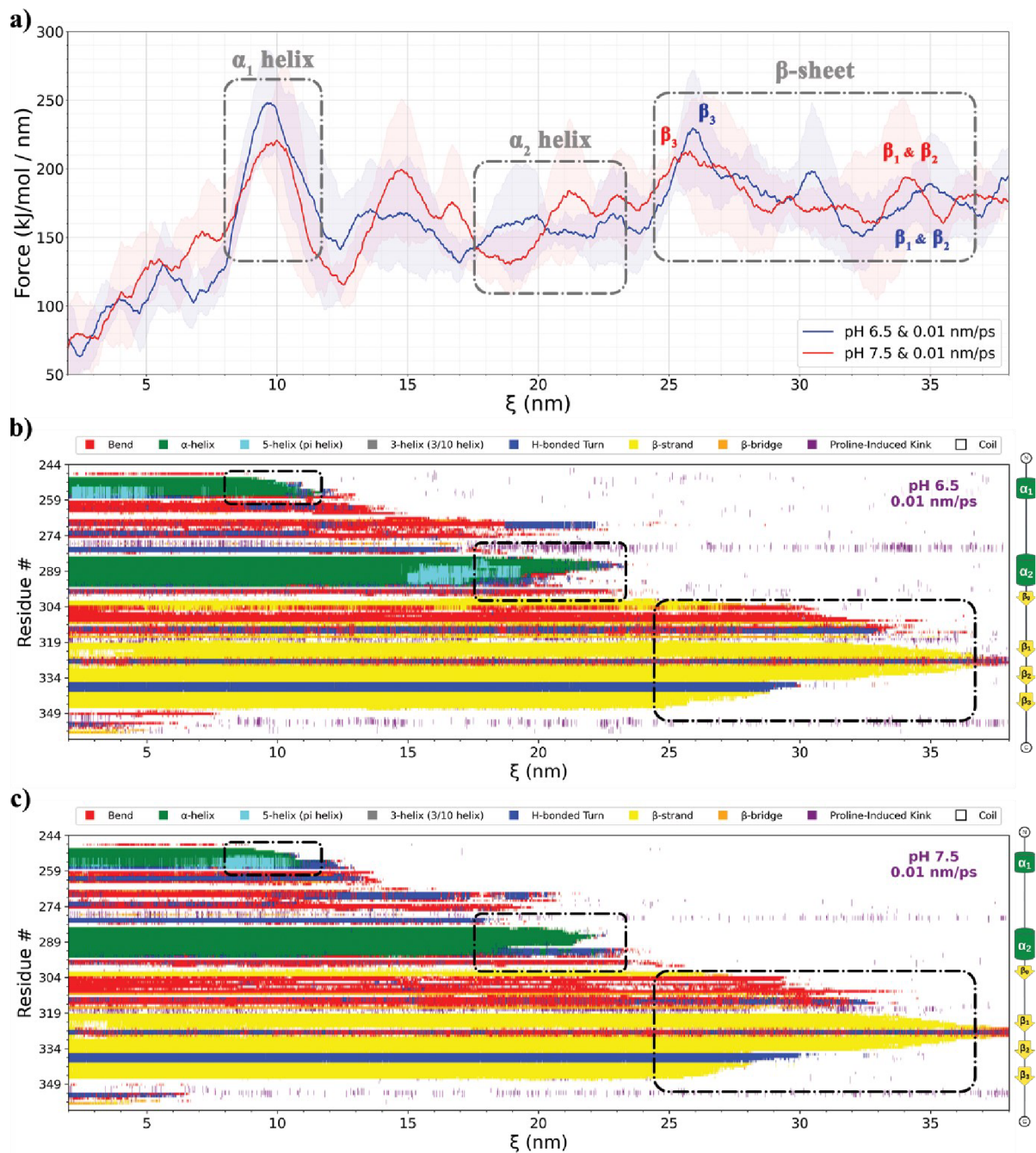
Figure 22: Analysis of Force and Structural Changes During Effector Domain Unfolding in Pulling Simulations. a) Force profiles as a function of the pulling distance, \xi (in nm), with the blue curve representing simulations at pH 6.5 and the red curve at pH 7.5, both at a pulling rate of 0.01 nm/ps. The shaded regions around each curve indicate the standard deviation, representing the variability within the force measurements for each average profile. Regions corresponding to \alpha_1 and \alpha_2 helices, and \beta -sheet are highlighted. b) & c) Derived from DSSP analysis, these plots detail the evolution of secondary structures along the effector domain sequence (residues) as it is extended, for pH 6.5 and 7.5 respectively. Key secondary structures are indicated by colour coding: green for \alpha -helices, yellow for \beta -strands, and other colours representing different structural motifs, illustrating the toxin's conformational changes over the simulation.
