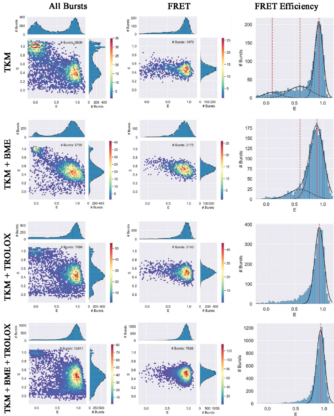
Figure 16: E-S (Efficiency vs. Stoichiometry) plots showcasing the FRET dynamics of the RNA hairpin across various buffer conditions. Each row represents a unique buffer mixture, with the first column showing the overall E-S plot for all observed bursts, the middle column focusing on FRET bursts, and the rightmost column depicting the FRET efficiency histograms. The density of points in E-S plots indicates the frequency of bursts with particular E and S values, while histograms illustrate the distribution of FRET efficiencies, with Gaussian fits overlaid to highlight the central tendencies under each condition.
