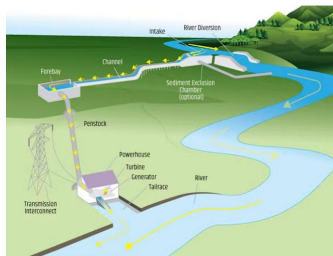
Figure 3.6: Schematic of run of river small hydro power plant (Source – US Department of Energy)
