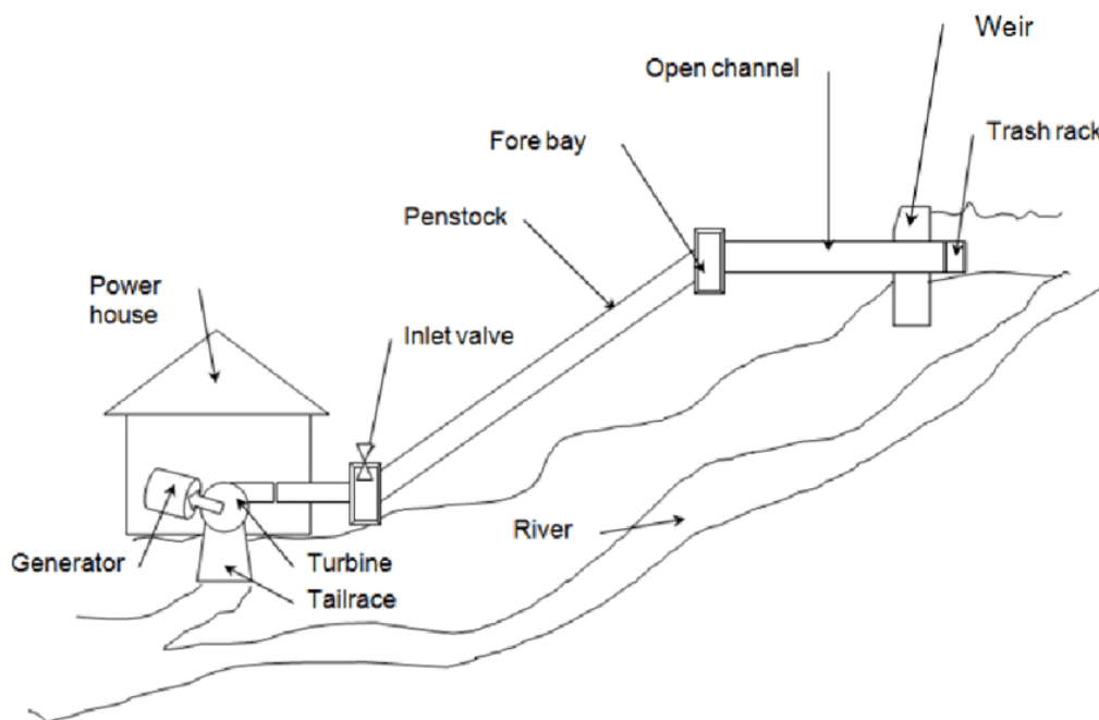
Figure 5.1: Working layout of Small Hydro Plant (Source – Energy.gov(Energy.Gov, 2022))
