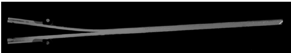
Figure 6.1: DCB specimen opening before crack growth
