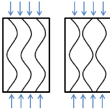
Figure 2.2: Fibre local buckling modes
