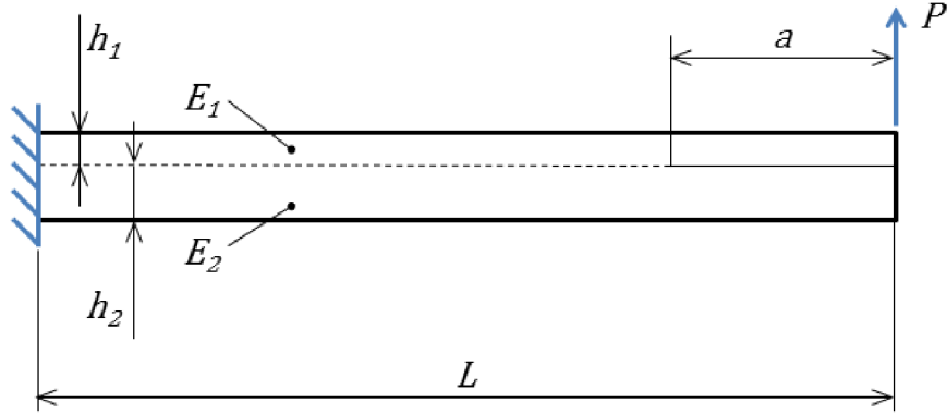
Figure 5.5: ADCB specimen
