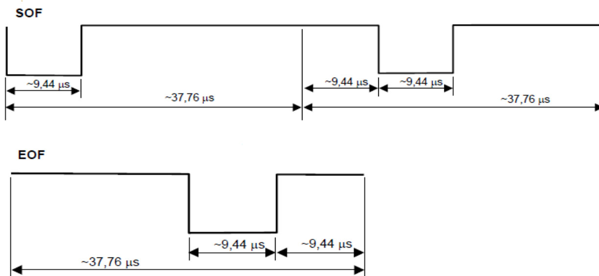
Obr. 3.6 – Formát SOF a EOF [22]
