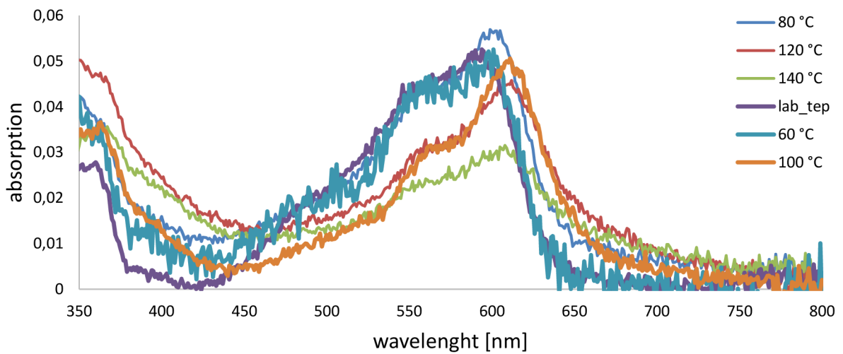
Figure 28 Plot of annealing in sample DPP U116.
