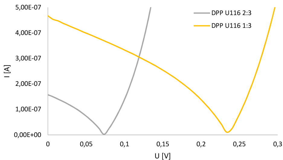
Figure 34 Plot of photocurrent DPP U115
